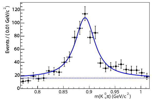
FIG. 3 (color online). Invariant mass of K_S^0 \pi^- combinations with all other analysis cuts applied. The solid curve is a Breit-Wigner line shape including detector resolution. The dotted line shows the combinatorial background.
