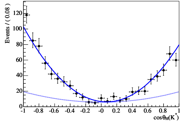
FIG. 2 (color online). Acceptance corrected distribution of \cos\theta_H(K^{*-}) . The solid line is a fit to a model which includes P -wave and S -wave interference as well as combinatorial background. The dotted line shows the combinatorial background estimated from the data.
