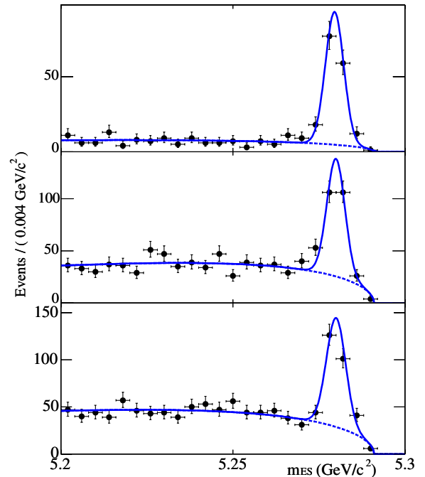
FIG. 1 (color online). Distributions of m_{\text{ES}} in the signal region for B^- \rightarrow D^0 K^{*-} decays where D^0 \rightarrow K^-\pi^+ (top), K^-\pi^+\pi^0 (middle), and K^-\pi^+\pi^-\pi^0 (bottom). The dashed curve indicates the contribution from the combinatorial background and the peaking B -background which is estimated from a simultaneous fit to the D^0 sideband (not shown).
