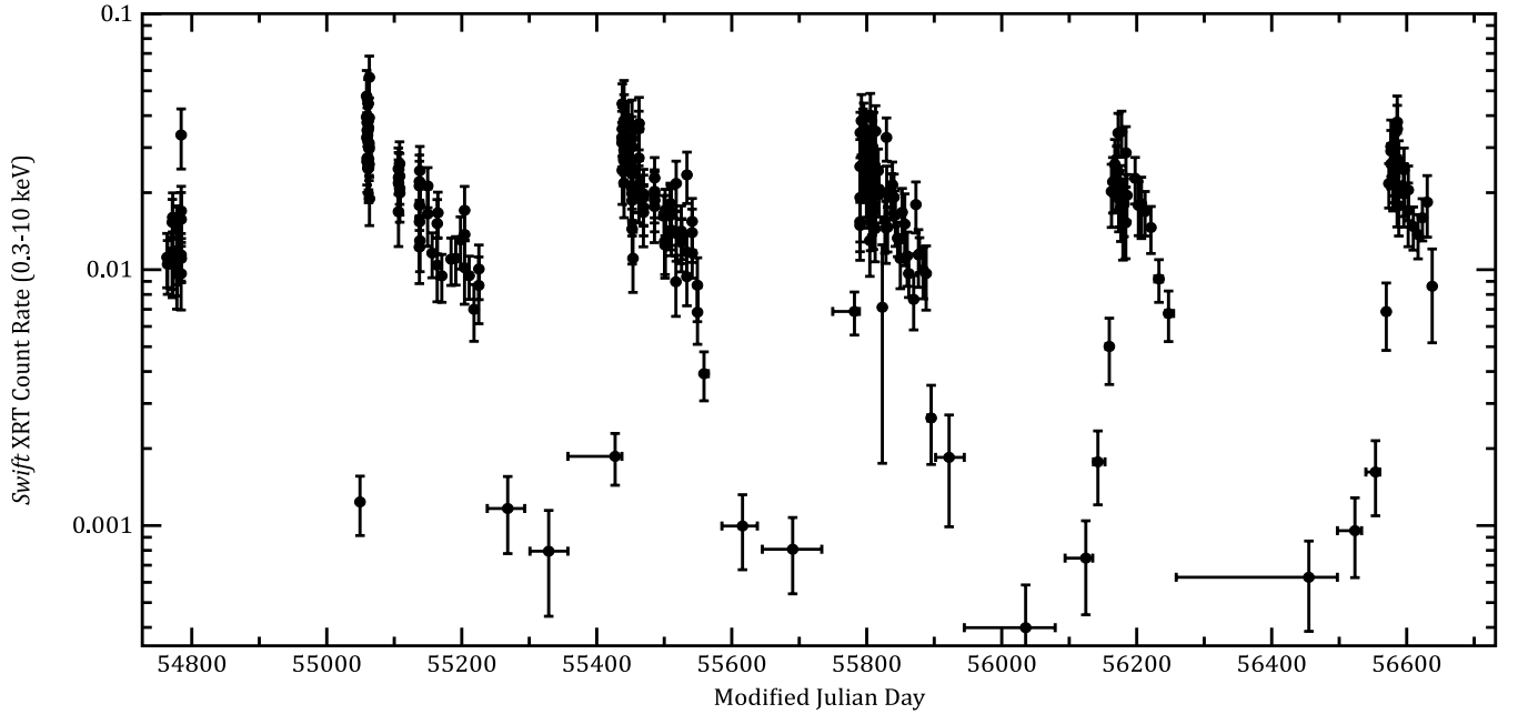
Figure 1. The Swift X-ray lightcurve of ESO 243-49 HLX-1 from 2008 until the end of 2013
