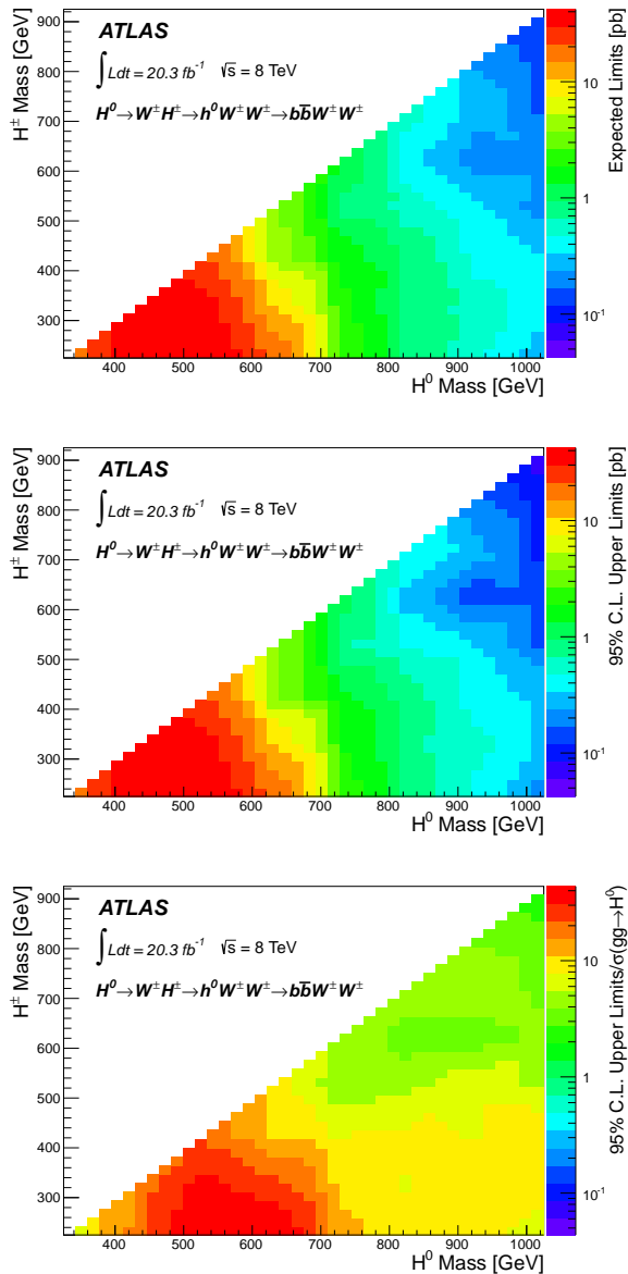
FIG. 6: The expected (top) and observed (middle) 95% C.L. upper limits on the cross section for gg \rightarrow H^0 \rightarrow W^\mp H^\pm \rightarrow W^\pm W^\mp h^0 \rightarrow W^\pm W^\mp b\bar{b} as a function of m_{H^0} and m_{H^\pm} . The ratio (bottom) of the observed 95% C.L. upper limits on the cross section to the theoretical cross section for a heavy Higgs boson produced via gluon-gluon fusion at the SM rate.
