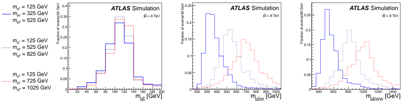
FIG. 2: Distributions of reconstructed masses in simulation for the three Higgs bosons in the cascade; the lightest Higgs boson, h^0 (left, as m_{bb} ), the charged Higgs boson, H^\pm (middle, as m_{b\bar{b}W} ), and the heavy Higgs boson, H^0 (right, as m_{b\bar{b}WW} ), shown for three example mass hypotheses.
