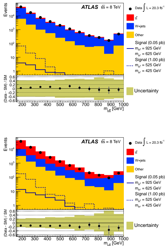
FIG. 3: Distributions of m_{b\bar{b}} with uncertainties in the control regions CR1 (top) and CR2 (bottom). The data (black points) are compared to the background model (stacked histogram). In control regions with fewer than two b -tagged jets, the two jets with the highest b -tagging scores are used. The final bin contains any overflow events. Two choices of signal hypotheses are also shown.
