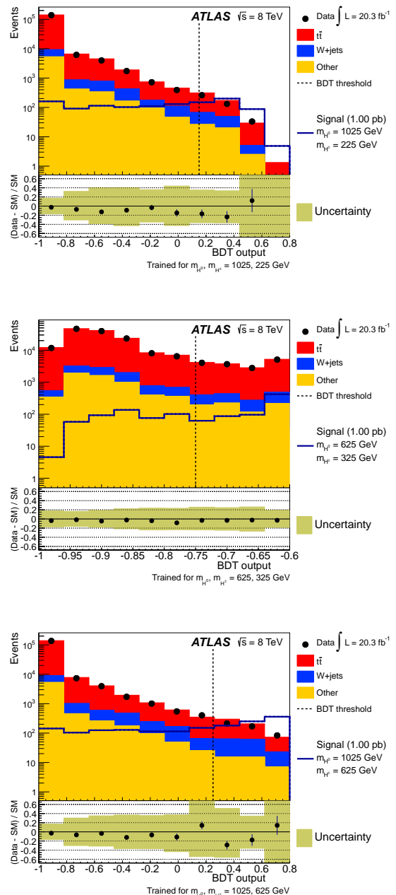
FIG. 5: Distributions of the BDT output in the signal regions for three example signal mass points, m_{H^0}, m_{H^\pm} = 1025, 225 GeV (top), m_{H^0}, m_{H^\pm} = 625, 325 GeV (middle), m_{H^0}, m_{H^\pm} = 1025, 625 GeV (bottom). Signal histograms have been scaled to a production cross section of 1 pb. BDT thresholds are shown as dashed lines for each mass point. The background model is shown as the coloured stacked histogram. The final bin contains any overflow events.
