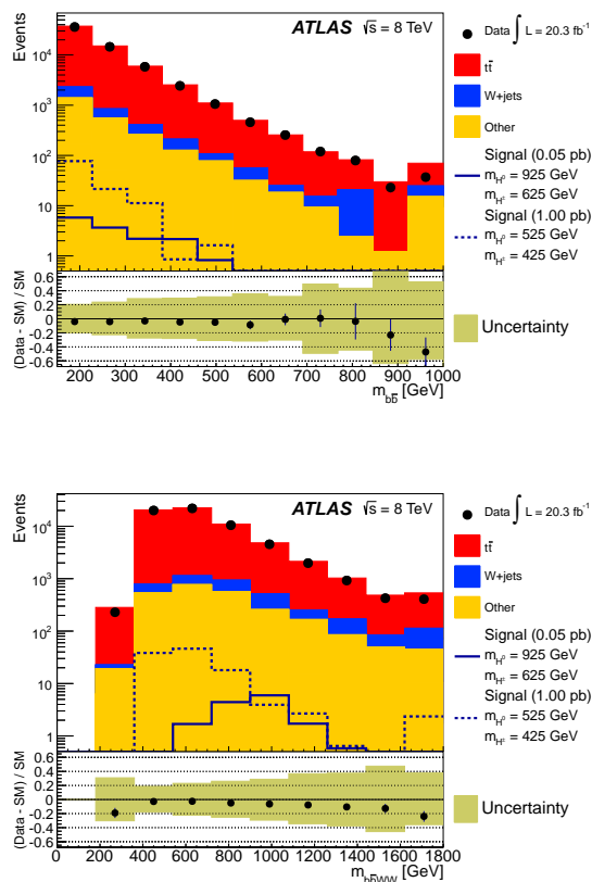
FIG. 4: Distributions of m_{b\bar{b}} (top) and m_{b\bar{b}WW} (bottom) with uncertainties in the control region CR3. The data (black points) are compared to the background model (stacked histogram). The final bin contains any overflow events. Two choices of signal hypotheses are also shown.
