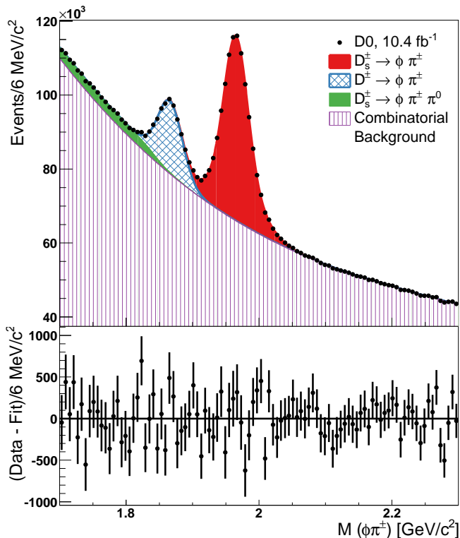
FIG. 1. The polarity-weighted \phi\pi^\pm invarient mass distribution. The lower mass peak is due to the decay D^\pm \rightarrow \phi\pi^\pm while the second peak is due to the D_s^\pm meson decay. Note the zero-suppression on the vertical axis. The bottom panel shows the fit residuals. The error bars represent the statistical uncertainties.
