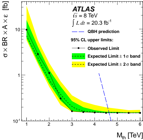
Figure 3: The 95% CL upper limits on \sigma \times BR \times A \times \epsilon for QBHs decaying to a photon and a jet, as a function of the threshold mass M_{\text{th}} , assuming M_D = M_{\text{th}} and n = 6 . The limits take into account statistical and systematic uncertainties. Points along the solid black line indicate the mass of the signal where the limit is computed. The black short dashed line is the central value of the expected limit. Also shown are the \pm 1\sigma and \pm 2\sigma uncertainty bands indicating the underlying distribution of possible limit outcomes under the background-only hypothesis. The predicted visible cross-section for QBHs is shown as the long dashed line.
