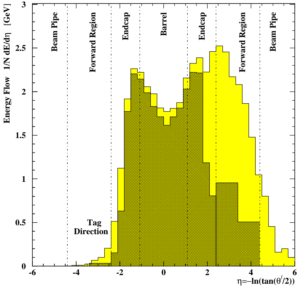
Figure 2: The hadronic energy flow per event based on the HERWIG generator as a function of the pseudorapidity \eta in the low- Q^2 region. The tagged electron is not shown. It is always at negative rapidities -3.5 < \eta < -2.8 . The dark shaded histogram represents the energy reconstructed by the OPAL detector after the simulation of the detector response to the HERWIG events. The vertical lines show the acceptance regions of the OPAL detector components. The generated energy distribution for these events is represented by the lightly shaded histogram.
