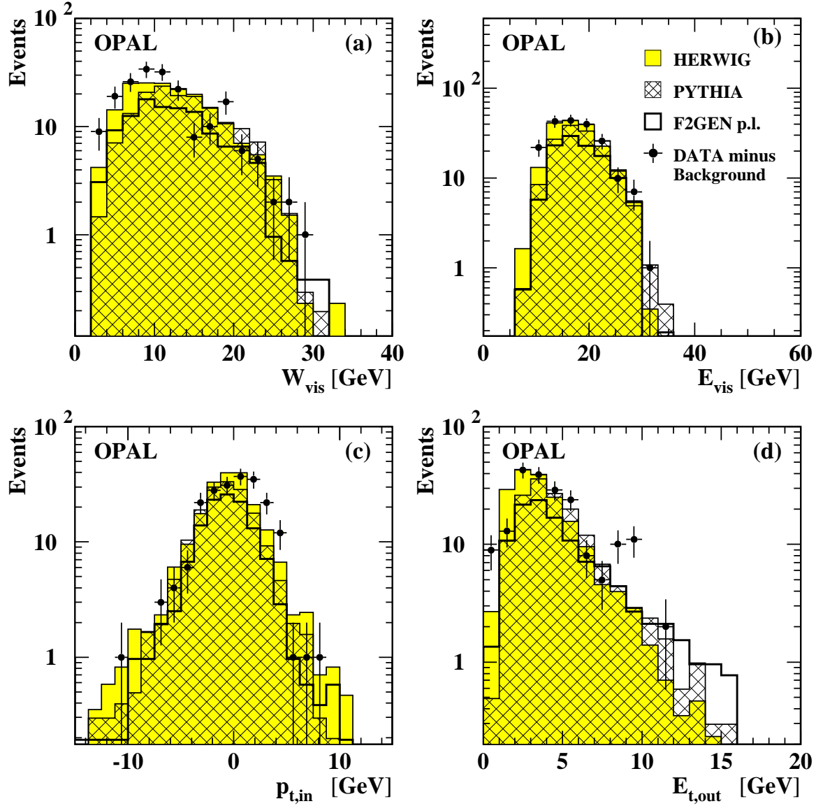
Figure 6: Comparison of data event quantities in the high- Q^2 region with HERWIG, PYTHIA and F2GEN pointlike (p.l.) Monte Carlo samples. (a) the distribution of the visible invariant mass, (b) the total visible energy of the event, (c) the transverse momentum of the event in the tag plane, (d) the energy out of the tag plane. The tag plane is defined by the beam direction and the direction of the tagged electron.
