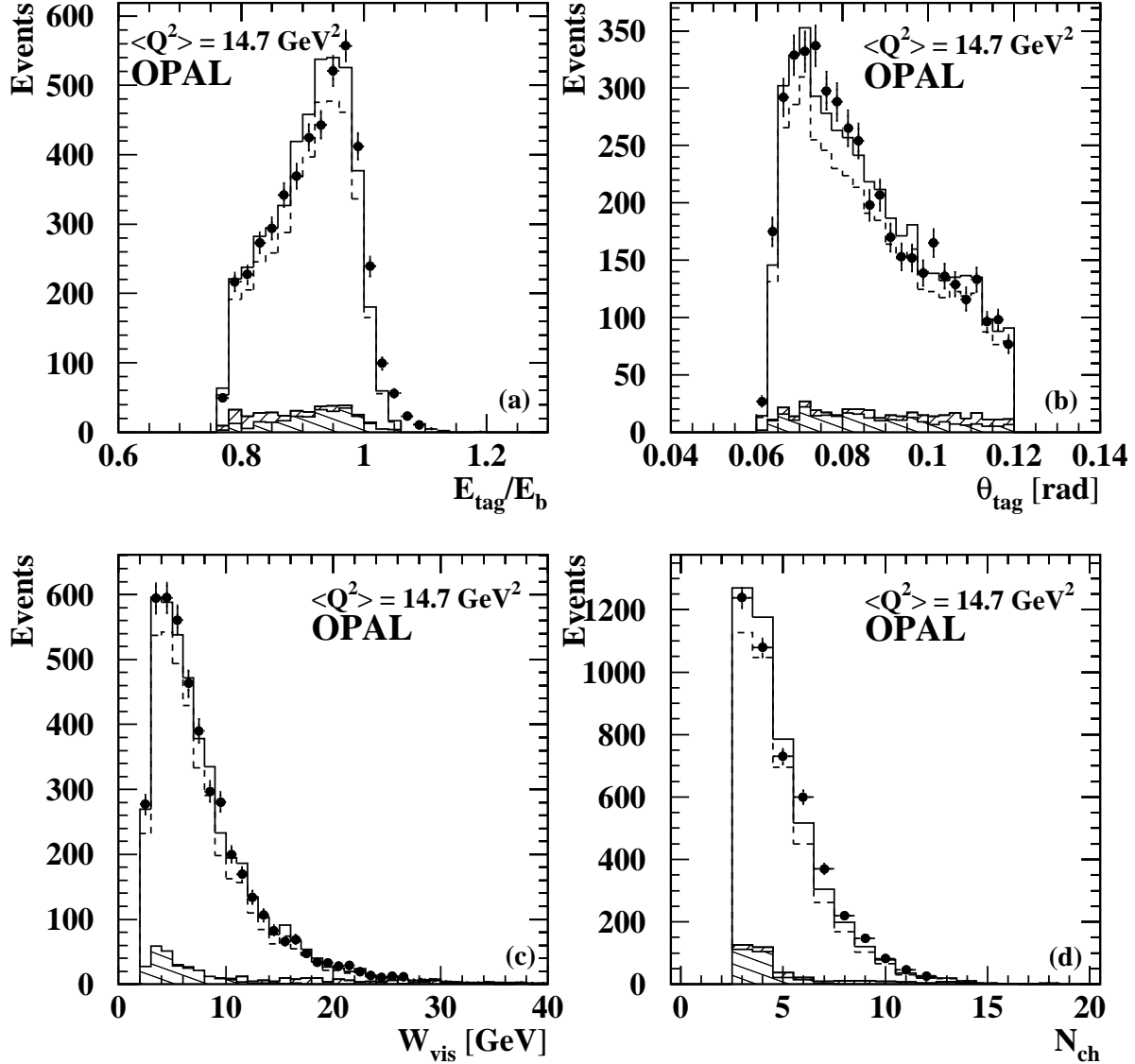
Figure 13: Distributions of measured quantities compared to the HERWIG Monte Carlo, using the GRV parametrisation and the standard cuts, for \langle Q^2 \rangle = 14.7 \text{ GeV}^2 . The variables shown are (a) the energy of the tagged electron as a fraction of the beam energy, (b) the polar angle of the tagged electron, (c) the visible invariant mass of the hadronic system, and (d) the number of charged particles seen in the detector. The meaning of the symbols is as defined in figure 12.
