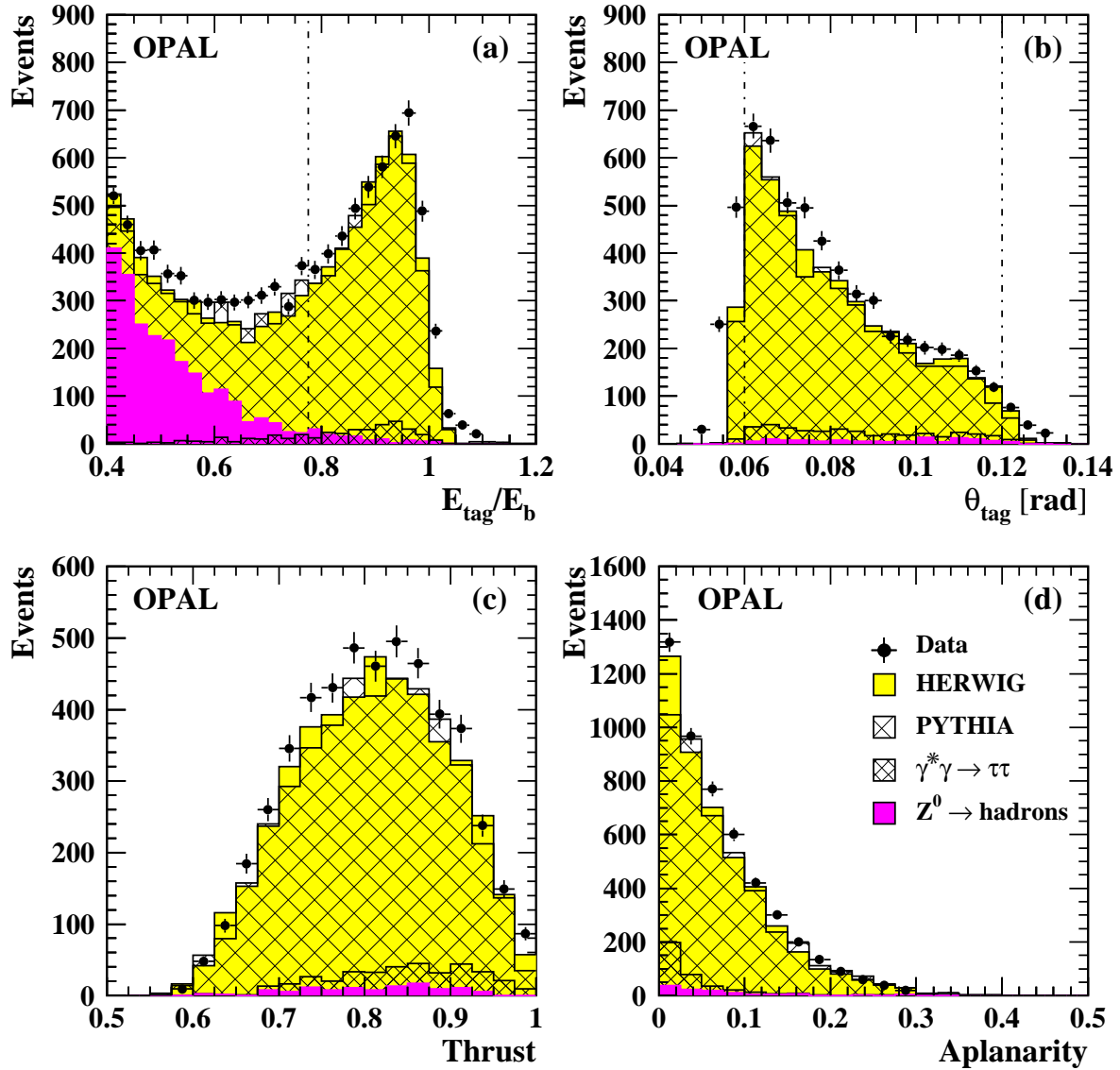
Figure 4: Comparison of data event quantities in the low- Q^2 region with the HERWIG and PYTHIA Monte Carlo models which have been normalised to the luminosity of the data. In figure (a) and (b) all cuts listed in section 3 are applied, except the one on the variable shown. In figures (c) and (d) all cuts are applied. The vertical lines in figure (a) and (b) indicate the cut values. The backgrounds from \gamma^*\gamma \rightarrow \tau^+\tau^- and Z^0 \rightarrow \text{hadrons} events, which are also shown separately at the bottom, have been added to the HERWIG and PYTHIA Monte Carlo samples. Thrust and aplanarity are calculated in the laboratory frame. All errors are statistical only.
