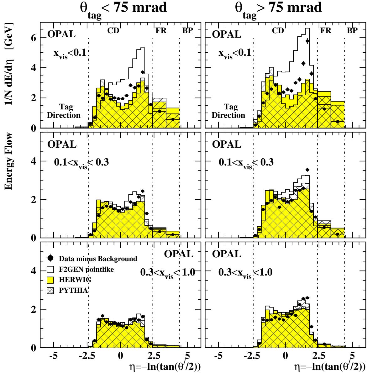
Figure 9: The hadronic energy flow per event as a function of pseudorapidity \eta for the data and various signal Monte Carlo samples. The energy flow is shown for various ranges of x_{\text{vis}} and \theta_{\text{tag}} for the low- Q^2 sample. The errors shown are statistical only. The vertical lines show the acceptance regions of the OPAL detector components. CD = Central Detector (including the barrel and endcaps), FR = Forward Region and BP = Beam Pipe.
