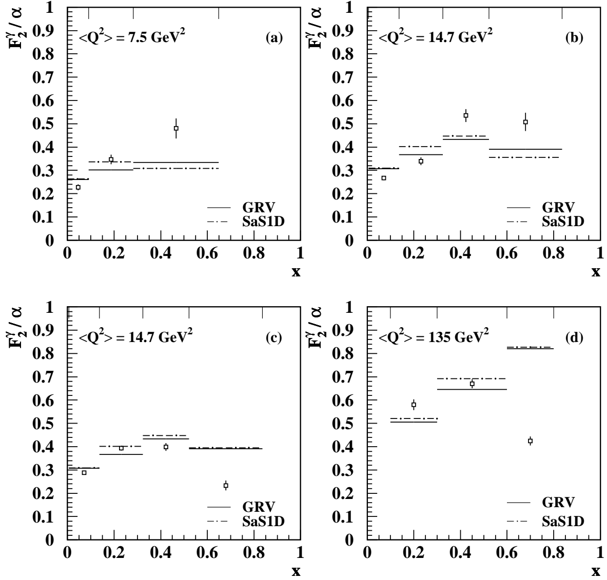
Figure 15: Unfolding tests using different Monte Carlo models to mimic the data (see text for further details). In (a) and (b) HERWIG, and in (c) and (d) PYTHIA are used to generate the mock data samples, always with the SaS1D parton density parametrisation. The model used to unfold the mock data is based on the reference sample as explained in the text. This sample uses the GRV parametrisation. The horizontal lines represent the mean F_2^\gamma of the samples in each bin. The dash-dotted lines represent the F_2^\gamma based on the SaS1D parton density parametrisation and the solid lines represent the F_2^\gamma based on the GRV parton density parametrisation. The points show the result of the unfolding of the mock data. The errors shown are statistical only. The vertical lines at the top of the figure indicate the bin sizes.
