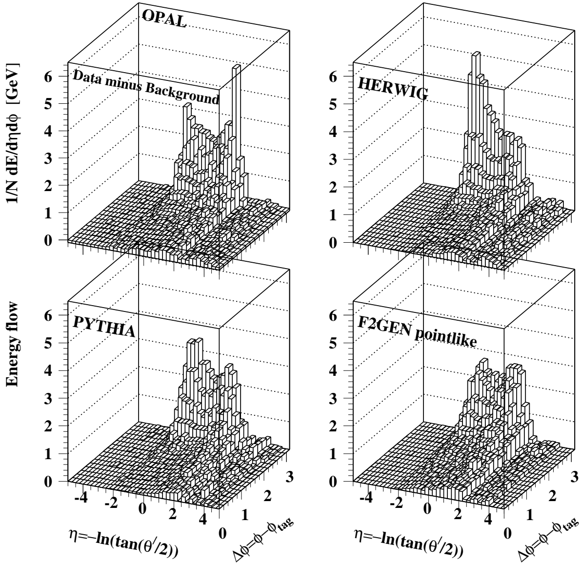
Figure 8: The hadronic energy flow per event in the low- Q^2 region as a function of pseudorapidity \eta and \Delta\phi . \theta' is the polar angle measured from the side opposite to the tagged electron, which is always at negative \eta and at \Delta\phi=0 .
