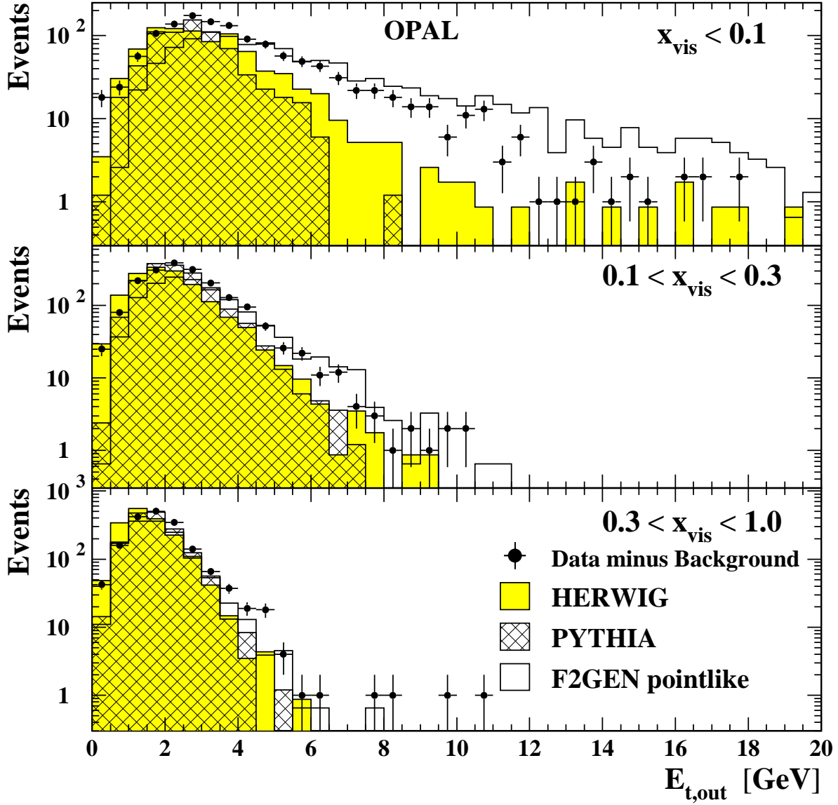
Figure 7: The energy transverse to the plane defined by the beam axis and the tag direction for three ranges in x_{\text{vis}} , for events in the low- Q^2 region.
