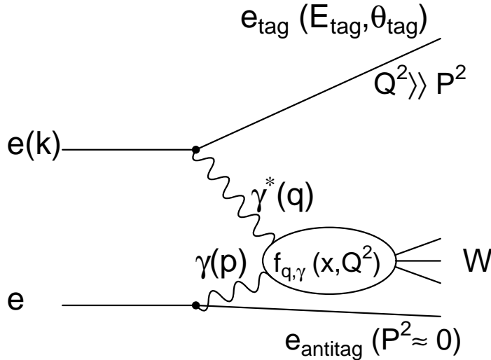
Figure 1: A diagram of deep inelastic electron-photon scattering.
