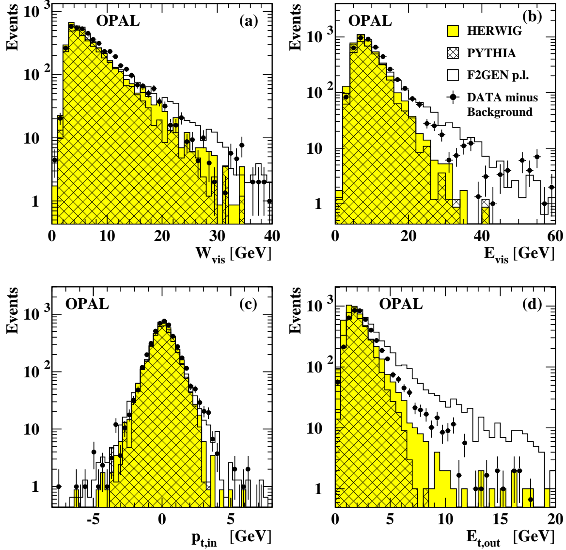
Figure 5: Comparison of data event quantities in the low- Q^2 region with HERWIG, PYTHIA and F2GEN pointlike (p.l.) Monte Carlo samples. (a) the distribution of the visible invariant mass, (b) the total visible energy of the event, (c) the transverse momentum of the event in the tag plane, (d) the energy out of the tag plane. The tag plane is defined by the beam direction and the direction of the tagged electron.
