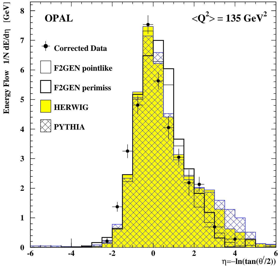
Figure 11: The measured energy flow per event in the high- Q^2 region, corrected for the detector inefficiencies, as a function of pseudorapidity \eta , compared to the generated energy flow of the HERWIG and PYTHIA Monte Carlo models and the energy flow of a sample of pointlike and perimiss events from the F2GEN model. The vertical error bars on the data points are the sum of the statistical and systematic errors, the horizontal bars indicate the bin widths. Note the different bin width in the forward regions.
