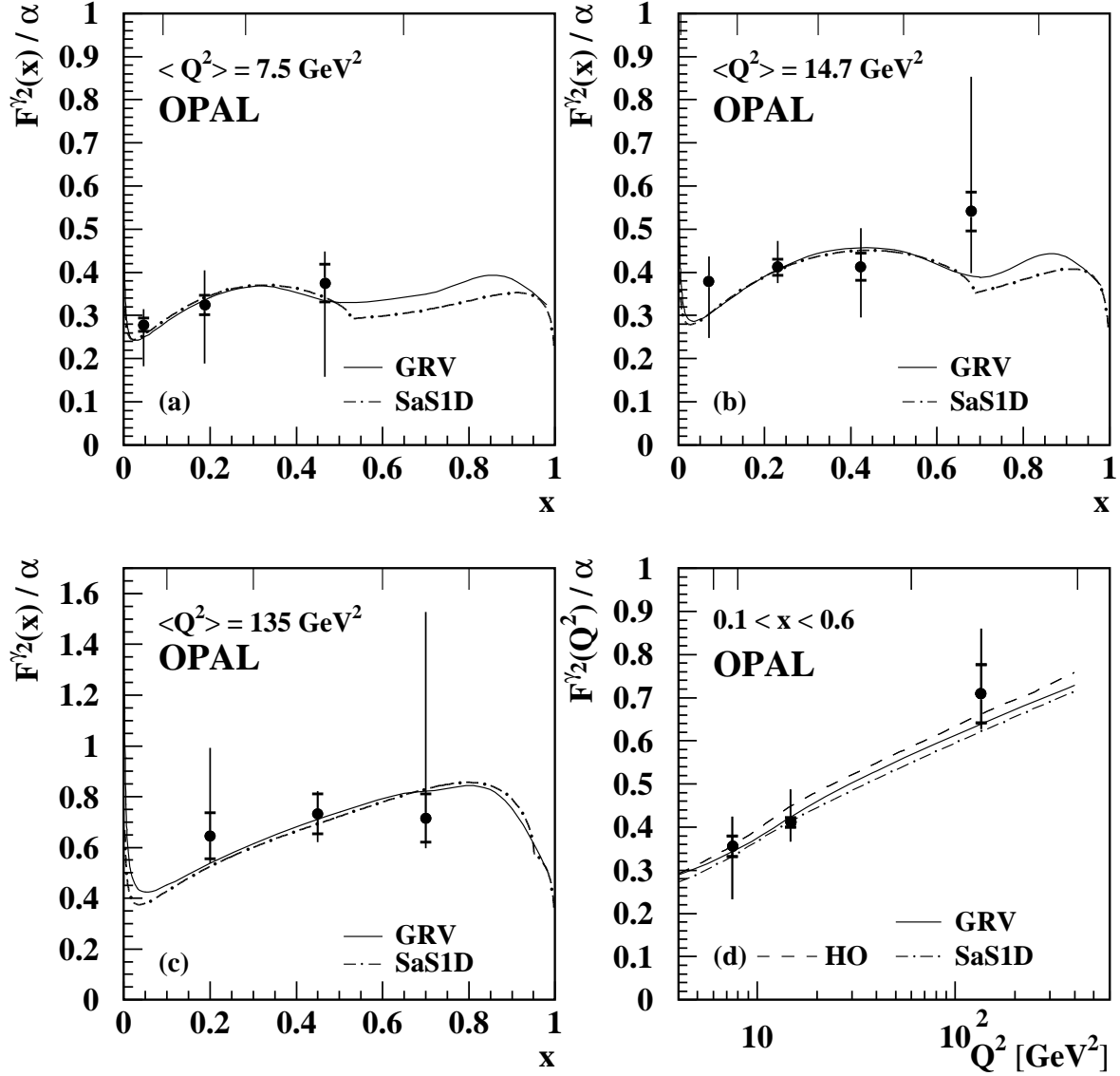
Figure 16: The measurement of F_2^\gamma for four active flavours for three values of \langle Q^2 \rangle , (a) \langle Q^2 \rangle = 7.5 \text{ GeV}^2 , (b) \langle Q^2 \rangle = 14.7 \text{ GeV}^2 , (c) \langle Q^2 \rangle = 135 \text{ GeV}^2 , and (d) the evolution of F_2^\gamma as a function of Q^2 for the x range 0.1 < x < 0.6 . The points show the measured F_2^\gamma . The bin sizes are indicated by the vertical lines at the top of the figure. The solid line represents the F_2^\gamma derived from the GRV parametrisation and the dash-dotted line denotes the F_2^\gamma derived from the SaS1D parametrisation, both using the Bethe-Heitler contribution to F_2^\gamma for massive charm quarks. The charm mass m_c is taken to be 1.3 GeV and 1.5 GeV in the case of SaS1D and GRV, respectively. The dashed curve labeled HO in (d) is a higher order prediction explained in the text.
