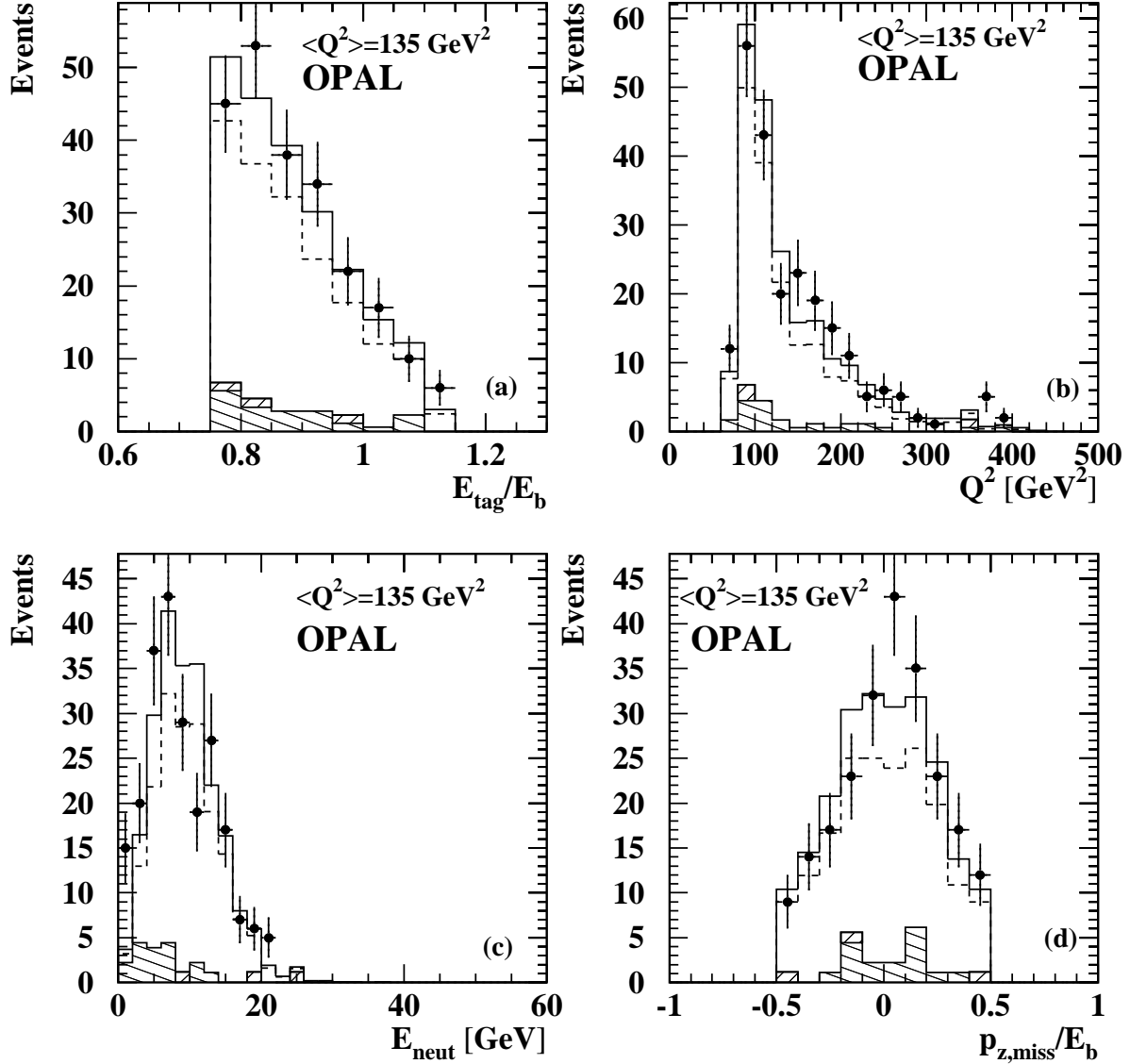
Figure 14: Distributions of measured quantities compared to the PYTHIA Monte Carlo, using the SaS1D parametrisation and the standard cuts, for \langle Q^2 \rangle = 135 \text{ GeV}^2 . The variables shown are (a) the energy of the tagged electron as a fraction of the beam energy, (b) the measured Q^2 , (c) the measured neutral energy, and (d) the missing longitudinal momentum of the event scaled by the beam energy. The meaning of the symbols is as defined in figure 12.
