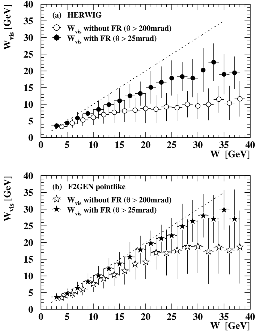
Figure 3: The correlation between the generated hadronic invariant mass W and the visible value W_{\text{vis}} with and without the hadronic energy sampled in the forward region (FR) of the OPAL detector. Figure (a) shows the correlation for HERWIG and (b) the correlation for F2GEN; in each case for two cuts on the minimum polar angle of the acceptance region. \theta > 25 mrad means that the energy of the forward region is included, whereas \theta > 200 mrad indicates that the detectors in the forward region are not used in the calculation of W_{\text{vis}} . The symbols show the average W_{\text{vis}} in each bin, and the vertical error bar its standard deviation. The dashed line represents W_{\text{vis}} = W .
