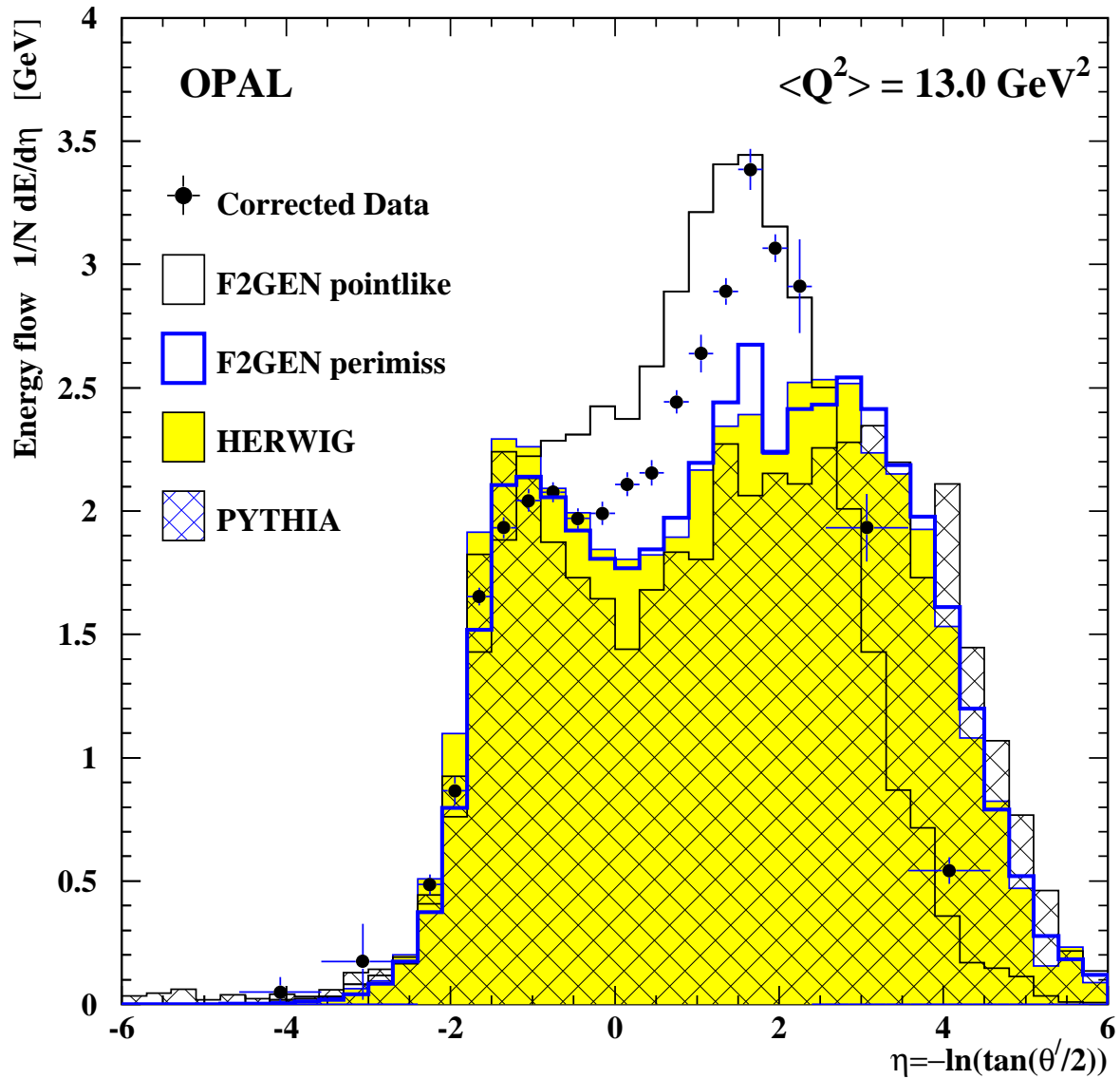
Figure 10: The measured energy flow per event in the low- Q^2 region, corrected for the detector inefficiencies, as a function of pseudorapidity \eta , compared to the generated energy flow of the HERWIG and PYTHIA Monte Carlo models and the energy flow of samples of pointlike and perimiss events from the F2GEN model. The vertical error bars on the data points are the sum of the statistical and systematic errors, and the horizontal bars indicate the bin widths. Note the different bin width in the forward regions.
