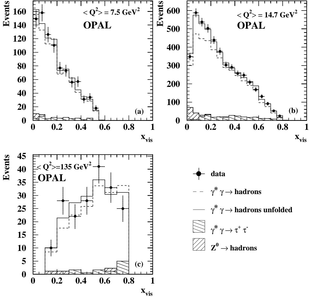
Figure 12: The distribution of x_{\text{vis}} for various mean momentum transfers \langle Q^2 \rangle . The dashed histogram shows the events from the HERWIG Monte Carlo, using the GRV parametrisation and the standard cuts, with the background events added to it, before the unfolding; the solid histogram shows the same quantity after the unfolding has been performed. The background events from \gamma^* \gamma \rightarrow \tau^+ \tau^- and Z^0 \rightarrow \text{hadrons} are also shown separately at the bottom of the figure. All errors shown are statistical only.
