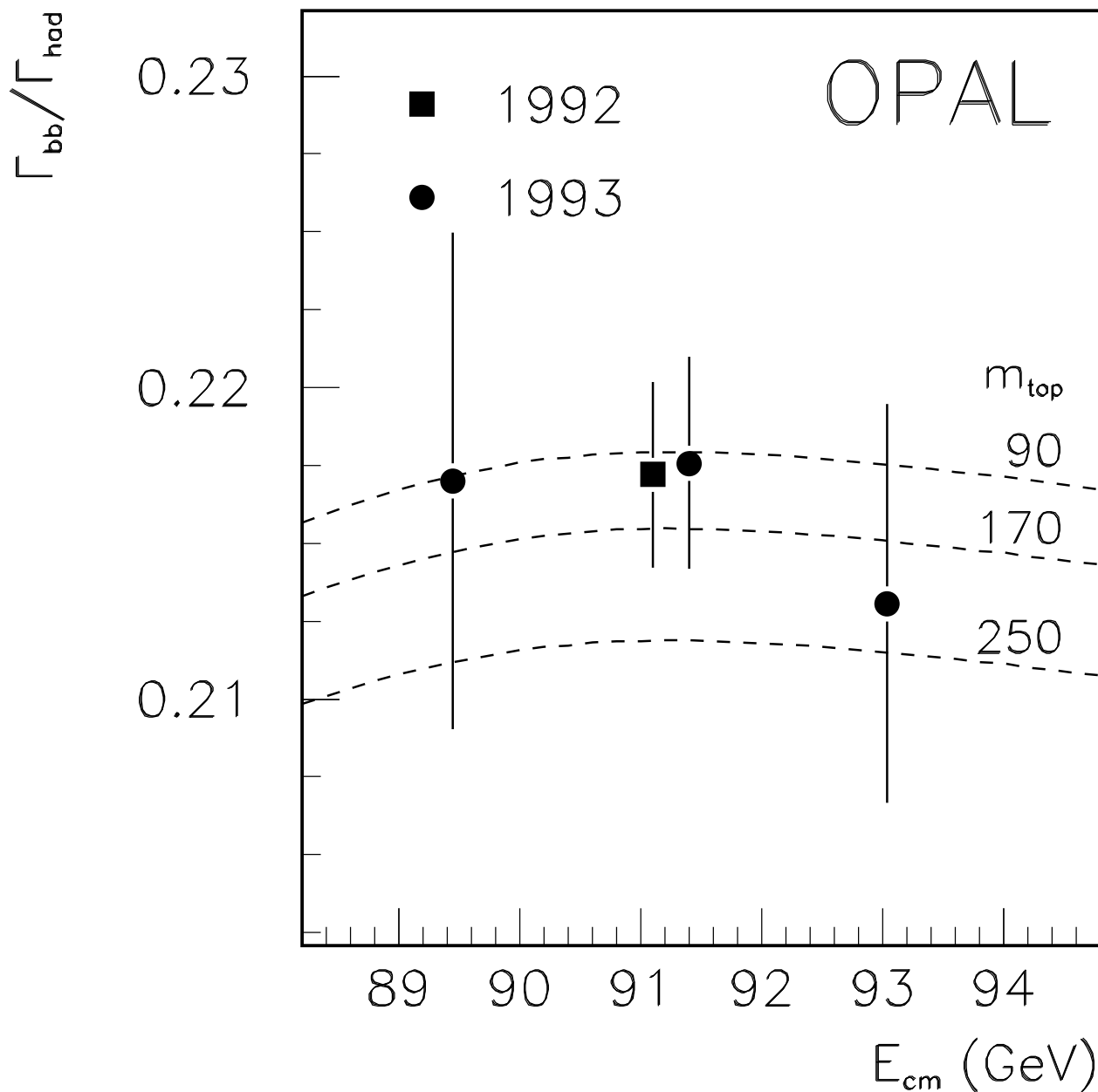
Figure 4: Values of \Gamma_{bb\bar{b}}/\Gamma_{had} obtained from data samples taken at different centre-of-mass energies E_{cm} . Errors are statistical. Points for 1992 and 1993 on-peak data are slightly shifted in E_{cm} . Dashed lines indicate the Standard Model prediction of the ratio \sigma(e^+e^- \rightarrow b\bar{b})/\sigma(e^+e^- \rightarrow hadrons) obtained using the ZFITTER program for top quark masses of 90, 170 and 250 \text{GeV}/c^2 , respectively from upper to lower. A value of m_{Higgs} = 300 \text{ GeV}/c^2 is assumed.
