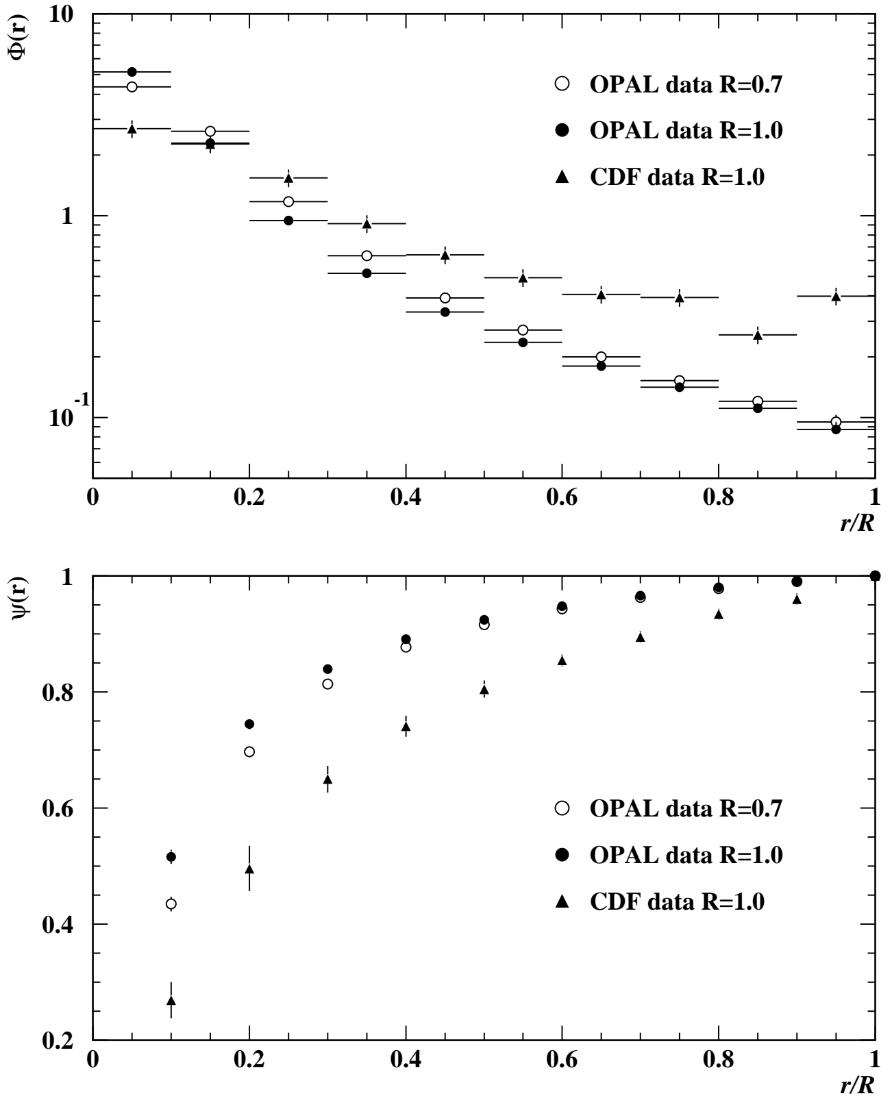
Figure 6: Energy profiles of jets defined using the cone jet finder, and having energy greater than 35 GeV. The data are shown for two values of the cone half-angle, R=0.7 rad and 1.0 rad, and use the E - \chi metric. Data from CDF are shown for comparison.
