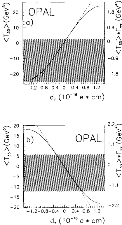
Fig. 2. Dependence of \langle T_{33} \rangle (left hand scale) on \vec{d}_\tau for \tau pair decays to (a) lepton-lepton and (b) hadron-hadron. The dashed line shows \langle T_{33} \rangle \cdot \Gamma(Z^0 \rightarrow \tau^+ \tau^-) (right hand scale). The shaded area represents the measured \langle T_{33} \rangle .
