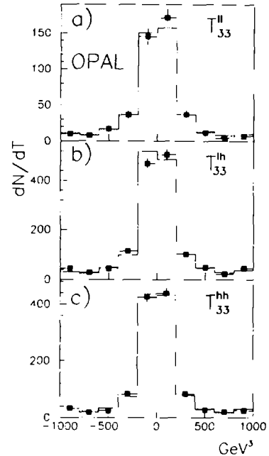
Fig. 1. T_{33} distributions for (a) the lepton-lepton, (b) the lepton-hadron, and (c) the hadron-hadron classes of events. Points with errors represent the data. The histogram (solid) represents the Monte Carlo expectation for \tilde{d}_\tau = 0 . The dotted lines are Monte Carlo expectations for (a) \tilde{d}_\tau = -10^{-16} e \text{ cm} and (b) \tilde{d}_\tau = 10^{-16} e \text{ cm} .
