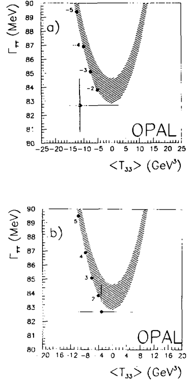
Fig. 3. The partial width \Gamma(Z^0 \rightarrow \tau^+ \tau^-) versus \langle T_{33} \rangle for (a) the lepton-lepton and (b) the hadron-hadron cases. \vec{d}_\tau ranges from 0 to 6 \times 10^{-17} e cm in this figure. The points correspond to the indicated values of \vec{d}_\tau in units of 10^{-17} e cm. The range for the width is due to the unknown top quark and Higgs boson masses and is indicated by the shaded area. The data point is the measured \langle T_{33} \rangle and partial width \Gamma(Z^0 \rightarrow \tau^+ \tau^-) [25].
