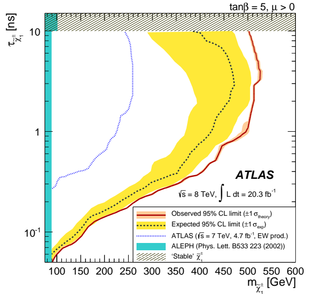
FIG. 6. The constraint on the allowed \tau_{\tilde{\chi}_1^\pm} - m_{\tilde{\chi}_1^\pm} space for \tan \beta = 5 and \mu > 0 . The black dashed line shows the expected limits at 95% CL, with the surrounding shaded band indicating the 1\sigma exclusions due to experimental uncertainties. Observed limits are indicated by the solid bold contour representing the nominal limit and the narrow surrounding shaded band is obtained by varying the cross-section by the theoretical scale and PDF uncertainties. The previous result from Ref. [8] and an example of the limits achieved at LEP2 by the ALEPH experiment [9] are also shown on the left by the dotted line and the shaded region, respectively. The search for charginos with long lifetimes, as indicated by the upper shaded region, is not covered by this analysis. The limits achieved at LEP2 by the ALEPH experiment of 101 GeV for long-lived charginos is taken from [9].
