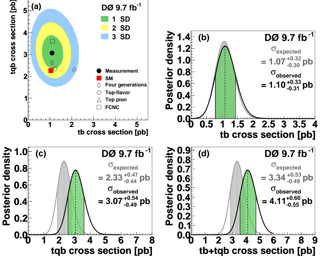
FIG. 4: (Color online.) Observed posterior density distributions extracted from the D_s^{\text{comb}} and D_t^{\text{comb}} discriminants: (a) 2D posterior density with one, two, and three SD probability contours, and the resulting 1D posterior densities for (b) the s channel, (c) the t channel, and (d) s+t channel, all along with expected posterior densities. The prediction from the SM [4] together with several BSM predictions are shown in (a), including four-quark generations with CKM matrix element |V_{ts}| = 0.2 [16], a top-flavor model with new heavy bosons with m_x = 1 TeV [46], a model of charged top-pions with m_{\pi^\pm} = 250 GeV [46], and flavor changing neutral currents with an up-quark/top-quark/gluon coupling \kappa_u/\Lambda = 0.036 [46, 47].
