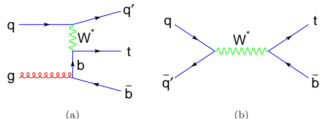
FIG. 1: (Color online.) Dominant lowest-order Feynman diagrams for (a) t -channel and (b) s -channel single top quark production.
