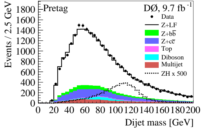
FIG. 5: (color online). Distribution of the dijet invariant mass, along with the background expectation, summed over all lepton channels in the pretag sample. The signal distribution, for M_H = 125 GeV, is scaled by a factor of 500.
