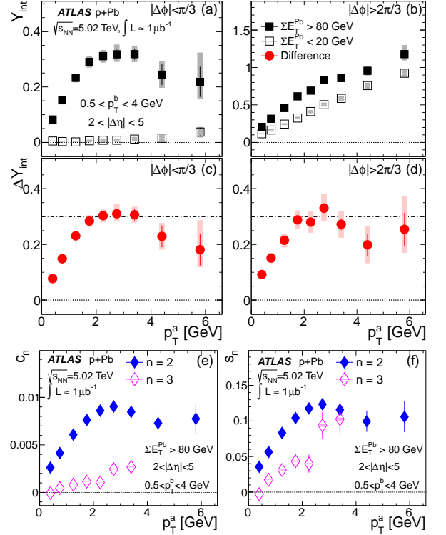
FIG. 4. Integrated per-trigger yields, Y_{\text{int}} (see text), vs p_T^a for 0.5 < p_T^b < 4 GeV in peripheral and central events, on the (a) near-side and (b) away-side. The panels (c) and (d) show the difference, \Delta Y_{\text{int}} . Panels (e) and (f) show the p_T dependence of c_n and s_n for n=2,3 , respectively. The error bars and shaded boxes represent the statistical and systematic uncertainties, respectively.
