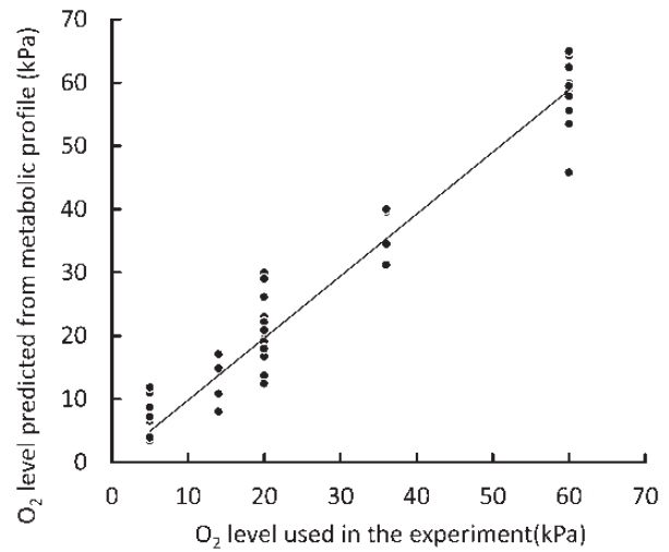
Fig. 5 Plot of measured versus PLS-R-predicted oxygen levels, showing a high correlation between observed and predicted oxygen levels (partial least squares regression; y = 0.981x ; R^2 = 0.944 , Q^2 [cross-validated] = 0.605, P < 0.001 [1000 random permutations]). Plot is based on nymphs at their critical thermal maxima only (treatments 1–3).
