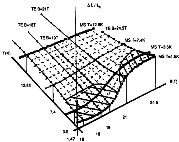
Fig. 4. Relative length change of the a -axis versus B in the interval 16\text{ T} < B < 24.5\text{ T} and versus T in the interval 1.5\text{ K} < T < 12.8\text{ K} as deduced from magnetostriction (MS) and thermal-expansion (TE) data. The type of experiment, the temperature and the field at which the experiments have been performed are indicated in the figure. Dashed areas indicate the regions with heavy-fermion-like features.
