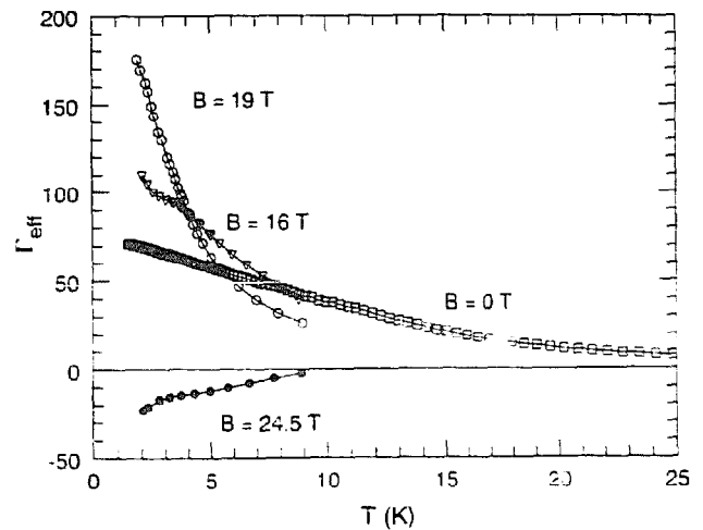
Fig. 3. Volume Grüneisen parameter for fields above and below B^* = 20 T as a function of temperature ( B \parallel a ).
