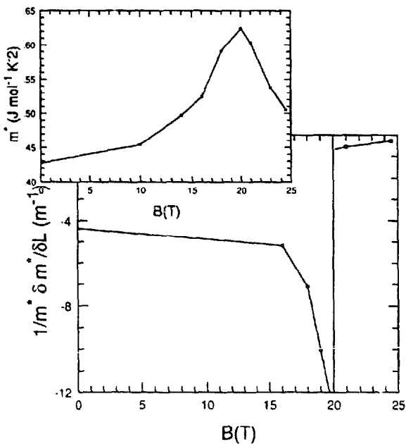
Fig. 2. Plot of the parameter \tau_a (-\partial \ln m^* / \partial x_a) , with x_a being the relative length change along the a -axis, as a function of field. The inset shows the field dependence of the coefficient of the linear term of the temperature dependence of the specific heat (taken from Ref. [2]) which is proportional to m^* .
