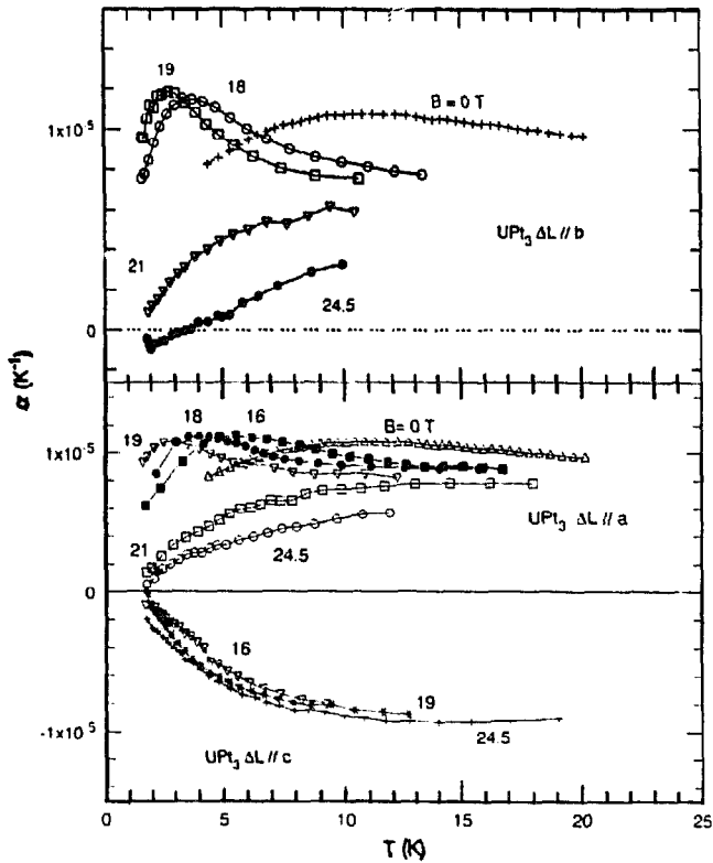
Fig. 1. Thermal expansion data ( B \parallel a ) in fields above and below B^* = 20 T along the crystallographic b -, a - and c -direction (from top to bottom).
