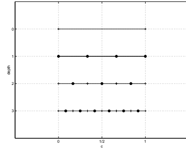
Figure 5: Depth of c by subdivision schema \mathcal{S} = [3, 2, 2]
