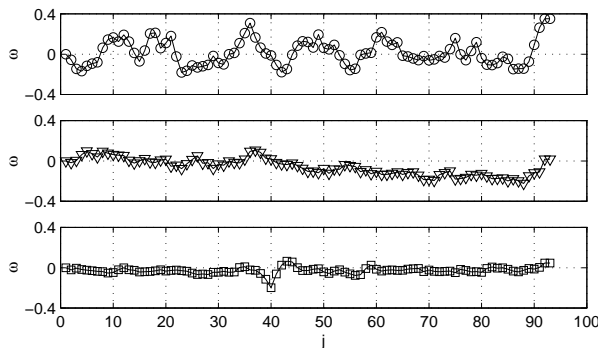
Figure 5: Examples of \omega sequences from the Beatles data set. From top to bottom, the sequences correspond to performances of a professional classical, amateur classical and professional jazz pianist. Each performance has different characteristics. For example the classical pianist uses a lot more tempo fluctuation than the professional jazz pianist. The amateur ‘rushes’, i.e. constantly accelerates.
