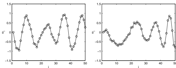
Figure 1: Typical “tempo curves” \omega that are sampled from Eq.2 with Q = 0.01I . Left, constant \theta = 0.5 , Right, \theta_i is interpolated linearly from 0.0 to 0.8 in 50 steps.
