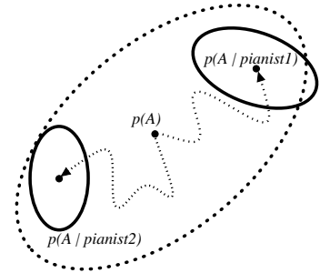
Figure 3: Online learning. The “big” ellipse represents a distribution over plausible parameters. The mean of this distribution corresponds to some average parameter setting, that is potentially sub-optimal for a particular pianist or performance situation. In online adaptation, parameter distributions drift to the “smaller” ellipses, eventually capturing the performer-specific parameter distribution.
