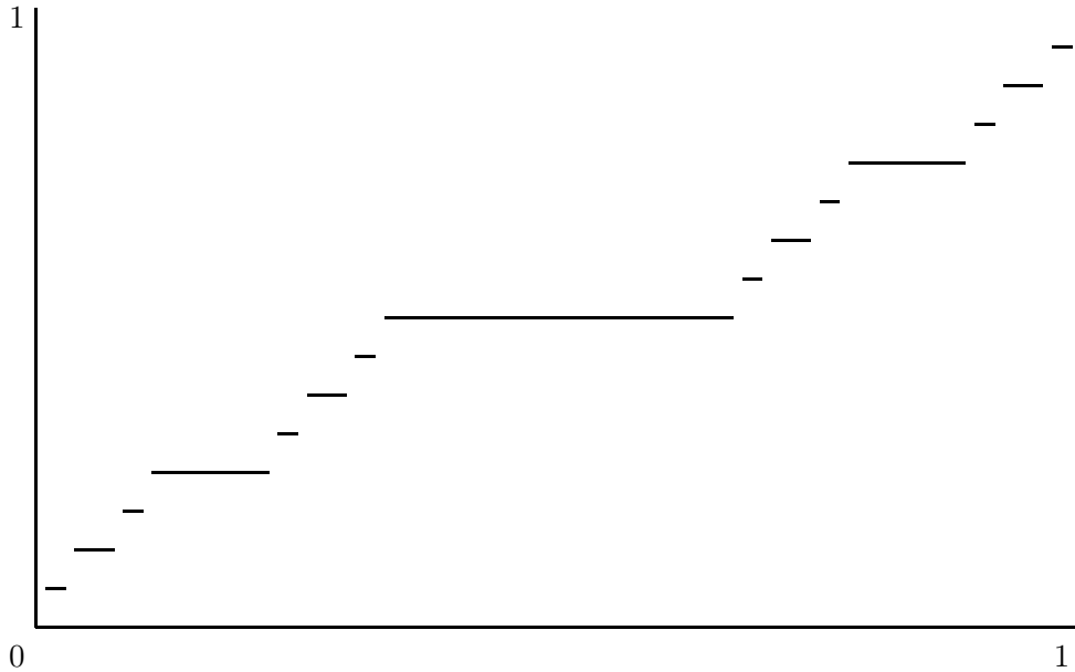
FIGURE 2.2. Cantor's function.
