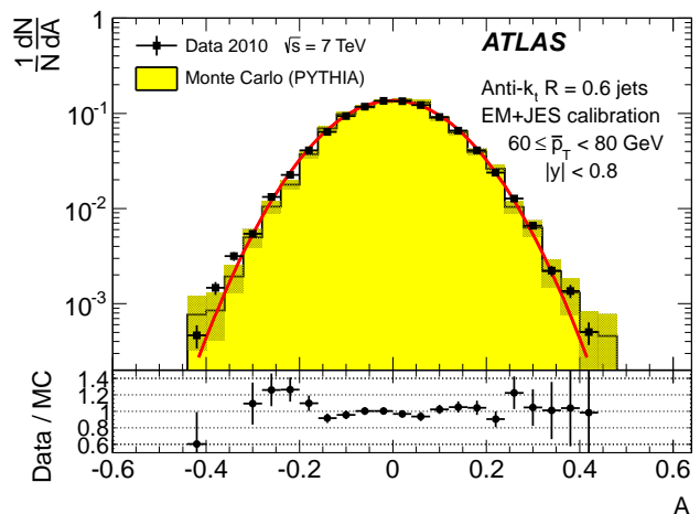
Fig. 1: Asymmetry distribution as defined in Equation (1) for \bar{p}_T = 60 - 80 \text{ GeV} and |y| < 0.8 . Data (points with error bars) and Monte Carlo simulation (histogram with shaded bands) are overlaid, together with a Gaussian fit to the data. The lower panel shows the ratio between data and MC simulation. The errors shown are only statistical.
