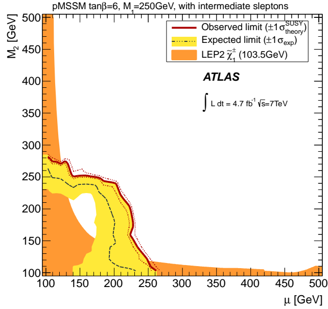
(c) M_1 = 250 GeV
