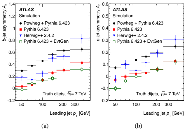
Fig. 3 The asymmetries in the amount of (a) bottom and (b) charm truth particle jets as taken from POWHEG+PYTHIA 6.423 (black points), PYTHIA 6.423 (squares), Herwig++ 2.4.2 (triangles) and PYTHIA+EVGEN (open squares) in leading and subleading jets, for each leading jet p_T bin used in the analysis.
