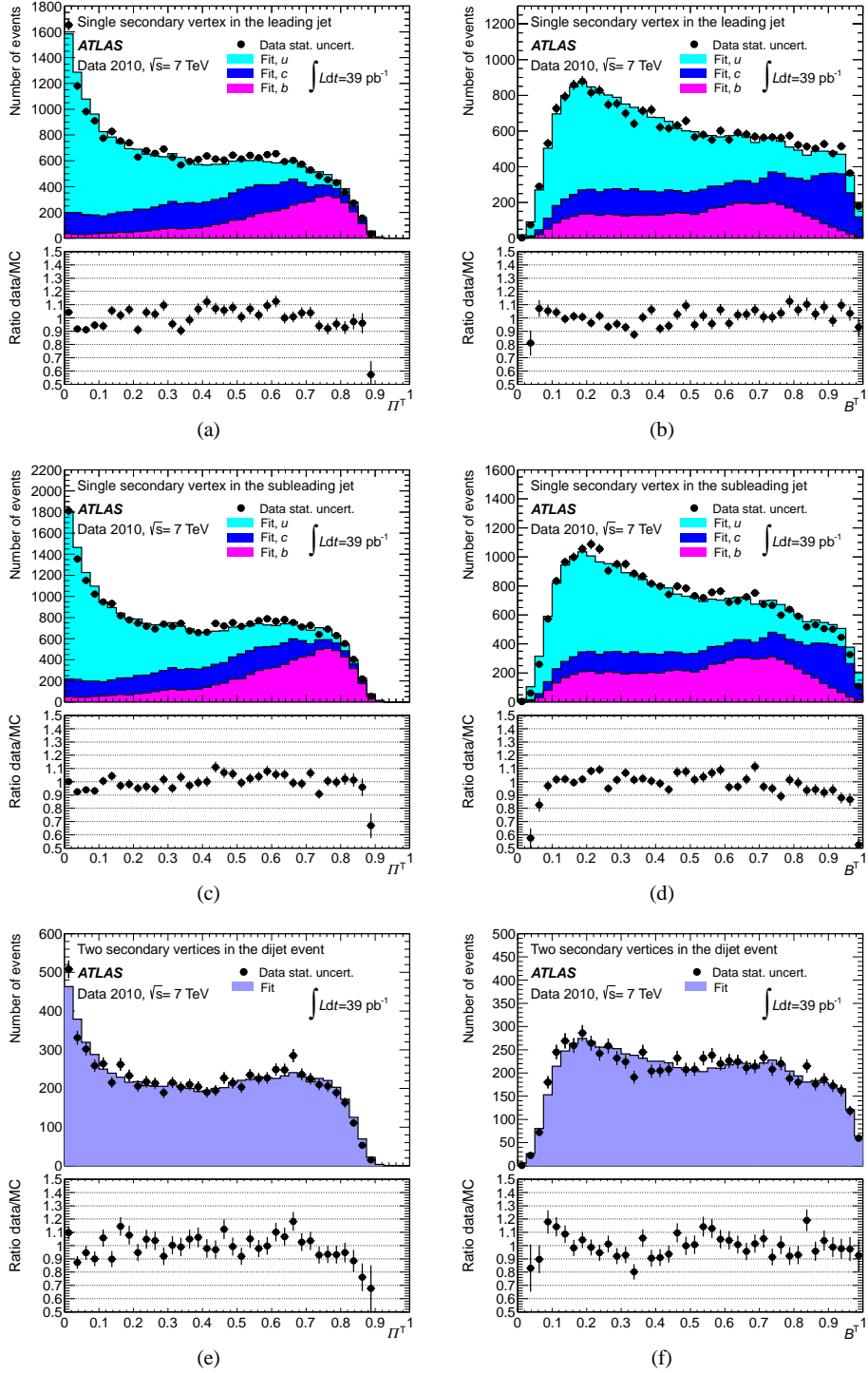
Fig. 8 Data description with the Monte Carlo templates obtained as a result of the fit in the [160,250] GeV analysis bin. (a) and (b) show the \Pi^T and B^T distributions for secondary vertices in the leading jet, (c) and (d) show the same distributions for secondary vertices in the subleading jet in events with a single secondary vertex in two jets. (e) and (f) show the \Pi^T and B^T distributions in the events with two secondary vertices averaged over leading and subleading jets. Data statistical uncertainties only are used to calculate the errors of the data to the Monte Carlo prediction ratios.
