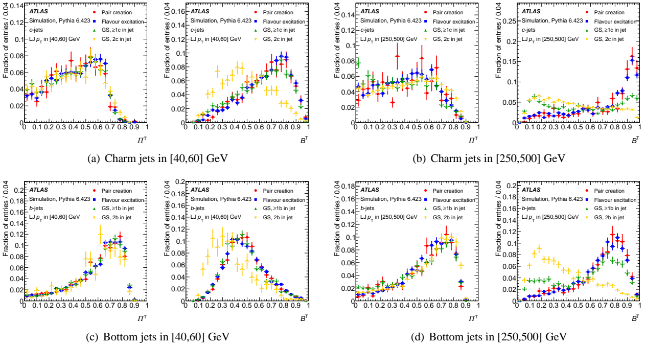
Fig. 7 The \Pi^+ and B^+ distributions in the [40, 60] GeV leading jet (LJ) p_T range for (a) charm jets and (c) bottom jets as well as in the [250, 500] GeV range for (b) charm jets and (d) bottom jets obtained with fully simulated PYTHIA 6.423 dijet events. The distributions are shown separately for jets stemming from quark pair creation, heavy flavour quark excitation, gluon splitting (GS) with one or two heavy flavour quarks inside the jet. All distributions are normalised separately to unit area.
