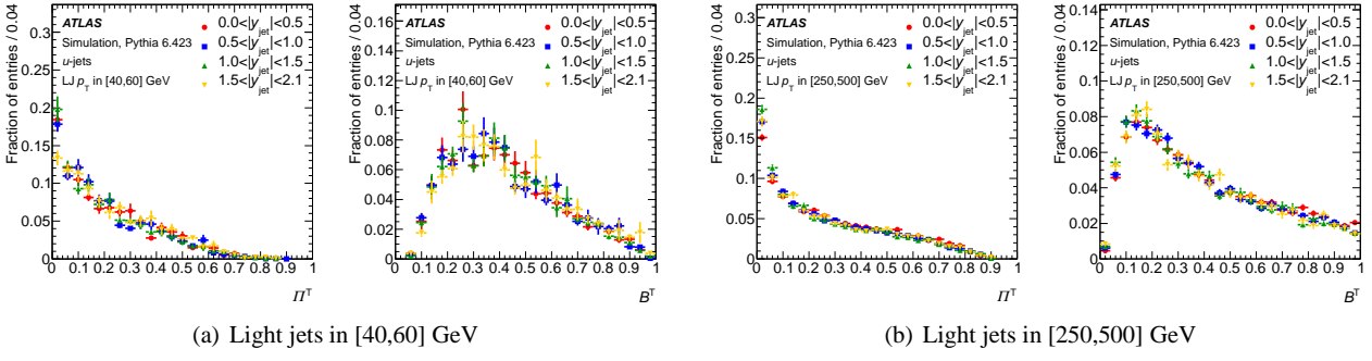
Fig. 6 The \Pi^+ and B^+ distributions of light jets in the (a) [40, 60] GeV and (b) [250, 500] GeV leading jet (LJ) p_T analysis bins obtained with fully simulated PYTHIA 6.423 dijet events. The distributions are shown in different jet rapidity ranges.
