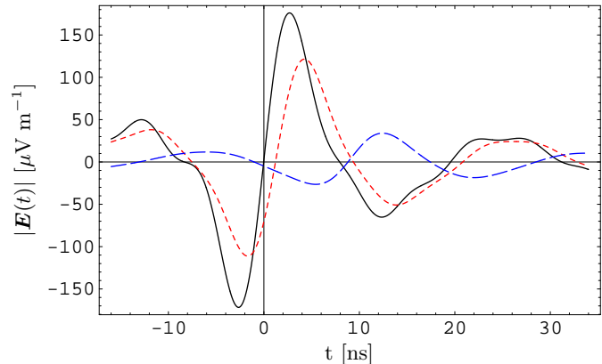
Fig. 15. Reconstructed pulses emitted by the maximum of a 10^{17} eV shower with flaring Agnetta et al. (1997) \Gamma -pdf, broken power-law energy distribution from \gamma = 5 –1000 and R_0 = 4 km, using an idealised rectangle filter spanning 40–160 MHz and “conservative \theta ” scenario. Solid: centre of illuminated area, short-dashed: 100 m from centre, dash-dotted: 250 m from centre
