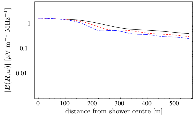
Fig. 12. Same as Fig. 10 but with “reduced \theta ” and magnetic field perpendicular to the direction of the observer.
