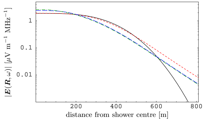
Fig. 7. Radial dependence of |E(\mathbf{R}, 2\pi 50 \text{ MHz})| for the maximum of a 10^{17} eV point source shower with R_0 = 4 km for the \gamma \equiv 60 case (solid) and for broken power-law distributions from \gamma = 5 –120 (short-dashed), \gamma = 5 –1000 (long-dashed) and \gamma = 5 –10000 (dash-dotted).
