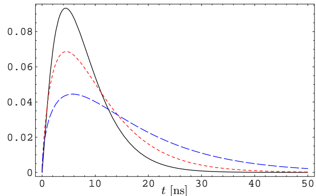
Fig. 4. \Gamma -pdf determining the arrival time distribution of particles as measured by Agnetta et al. (1997). Solid: in the shower centre, short-dashed: 50 m from shower centre, long-dashed: 100 m from shower centre.
