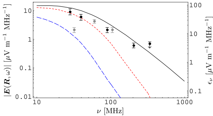
Fig. 16. |E(\mathbf{R}, 2\pi\nu)| -spectrum of a full 10^{17} eV air shower with flaring Agnetta et al. (1997) \Gamma -pdf, “conservative \theta ” approach, R_0 = 4 km and a broken power-law energy distribution from \gamma = 5 –1000. Solid: centre of illuminated area, short-dashed: 100 m from centre, long-dashed: 250 m from centre, black points: rescaled Spencer (1969) data as presented by Allan (1971), grey points: rescaled Prah (1971) data
