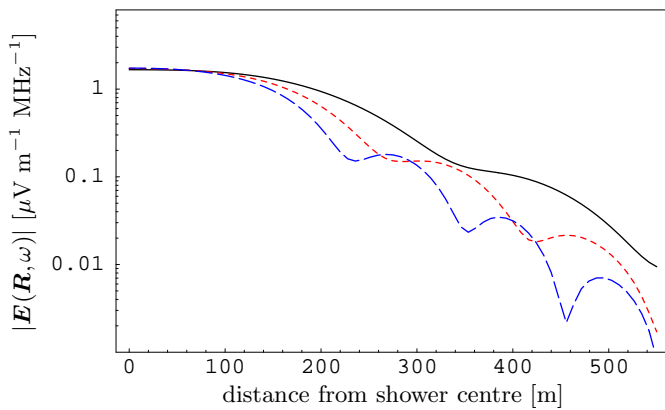
Fig. 10. Radial dependence of |E(\mathbf{R}, 2\pi\nu)| for the maximum of a 10^{17} eV air shower with full longitudinal coherence, realistic lateral structure, “conservative \theta ” approach, R_0 = 4 km and a broken power-law energy distribution from \gamma = 5 –1000. Solid: \nu = 50 Mhz, short-dashed: \nu = 75 Mhz, long-dashed: \nu = 100 Mhz
