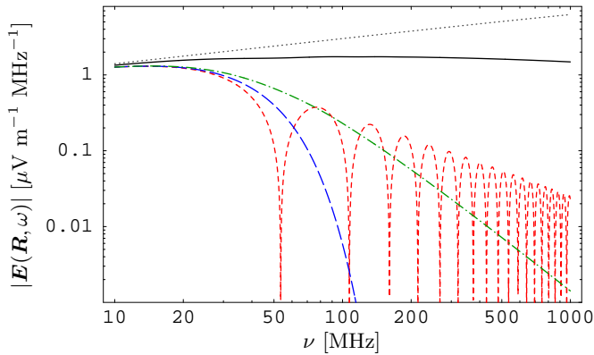
Fig. 9. |E(\mathbf{R}, 2\pi\nu)| -spectrum at the centre of the area illuminated by the maximum of a 10^{17} eV air shower with realistic lateral distribution, R_0 = 4 km and a broken power-law energy distribution from \gamma = 5 –1000. Solid: full longitudinal coherence, short-dashed: uniform 5.6 m longitudinal distribution, long-dashed: Gaussian longitudinal distribution with \sigma = 1.61 m, dash-dotted: longitudinal \Gamma -distribution with c\sigma_t = 1.61 m. For comparison: fully coherent case without lateral distribution (dotted)
