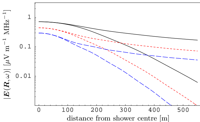
Fig. 14. Radial dependence of |E(\mathbf{R}, 2\pi\nu)| for the maximum of a 10^{17} eV air shower with flaring Agnetta et al. (1997) \Gamma -pdf, R_0 = 4 km and a broken power-law energy distribution from \gamma = 5 –1000. Solid: \nu = 50 MHz, short-dashed: \nu = 75 MHz, long-dashed: \nu = 100 MHz, upper/lower curves for “reduced \theta ” perpendicular/parallel to magnetic field direction
