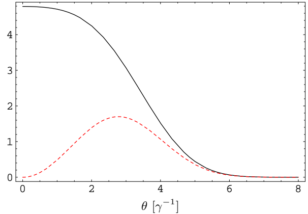
Fig. 3. Comparison of |A_{\parallel}| (solid) and |A_{\perp}| (short-dashed) for \nu = 100 MHz, \gamma = 60 and B = 0.3 G. Absolute scale is arbitrary.
