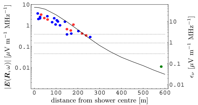
Fig. 17. Radial dependence of |E(\mathbf{R}, 2\pi 55 \text{ MHz})| for a full 10^{17} eV air shower with flaring Agnetta et al. (1997) \Gamma -pdf, “conservative \theta ” approach, R_0 = 4 km and a broken power-law energy distribution from \gamma = 5 –1000, data from Allan et al. (1970), horizontal lines from top to bottom: emission strength needed for a 3\sigma -detection with an individual LOPES antenna or an array of 10 or 100 LOPES antennas
