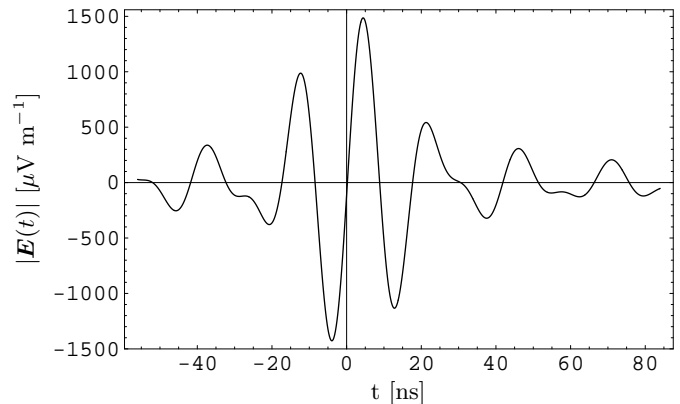
Fig. 18. Reconstructed pulse in the centre of the area illuminated by a full 10^{17} eV shower with flaring Agnetta et al. (1997) \Gamma -pdf, broken power-law energy distribution from \gamma = 5 –1000 and R_0 = 4 km, using an idealised rectangle filter spanning 42.5–77.5 MHz
