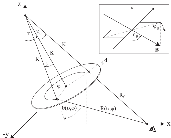
Fig. 8. The geometry for the air shower maximum.
