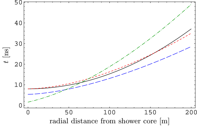
Fig. 5. Radial dependence of the particle arrival time distribution. Solid: shower curvature as given by a spherical surface with K = 2,300 m, short-dashed: \langle t \rangle(r) as given by Agnetta et al. (1997), long-dashed: \sigma_t(r) as given by Agnetta et al. (1997), dash-dotted: \sigma_{t,L}(r) as given by Linsley (1986).
