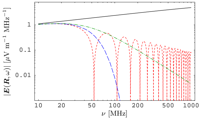
Fig. 6. |E(\mathbf{R}, 2\pi\nu)| -spectrum in the centre of the area illuminated by the maximum of a 10^{17} eV air shower with R_0 = 4 km and \gamma \equiv 60 . Solid: full coherence, short-dashed: uniform 5.6 m line charge, long-dashed: Gaussian line charge with \sigma = 1.61 m, dash-dotted: asymmetrical \Gamma -distribution with c\sigma_t = 1.61 m
