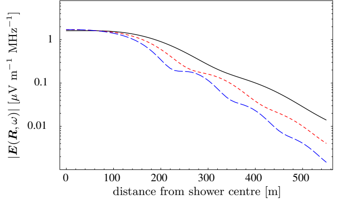
Fig. 11. Same as Fig. 10 but with “reduced \theta ” and magnetic field parallel to the direction of the observer.
