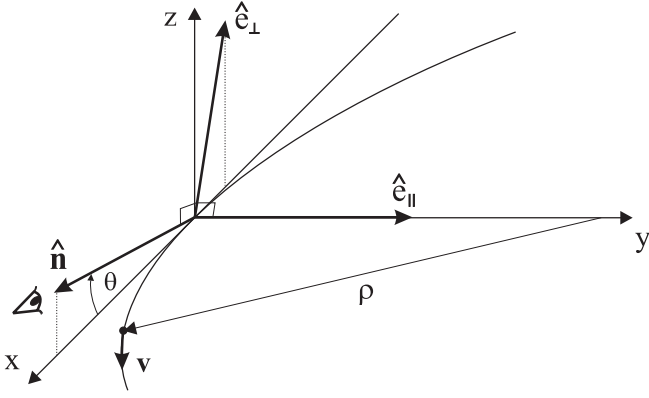
Fig. 1. Geometry of single particle synchrotron radiation for an observer with line-of-sight vector \hat{\mathbf{n}} enclosing a minimum angle \theta to the instantaneous particle velocity vector \mathbf{v} . The equivalent curvature radius is given by \rho , and the emission can be conveniently divided into the components \hat{\mathbf{e}}_{\perp} and \hat{\mathbf{e}}_{\parallel} . The particle trajectory lies in the x-y plane.
