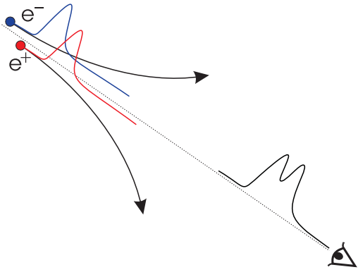
Fig. 2. Misalignment between the electron and the positron in an electron-positron pair no longer allows coherent addition of the individual emissions.
