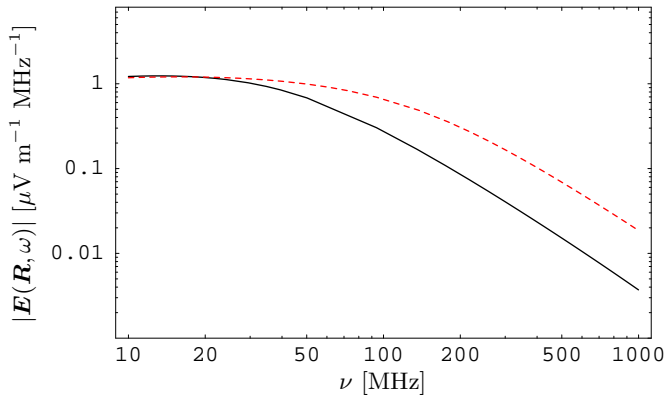
Fig. 13. |E(\mathbf{R}, 2\pi\nu)| -spectrum at the centre of the area illuminated by the maximum of a 10^{17} eV air shower with flaring \Gamma -pdf, R_0 = 4 km and a broken power-law energy distribution from \gamma = 5 –1000. Solid: flaring Agnetta et al. (1997) lateral distribution, short-dashed: flaring Linsley (1986) lateral distribution
