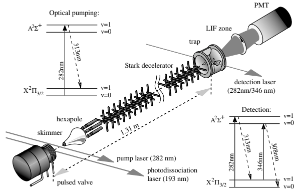
FIG. 1. Scheme of the experimental setup. A pulsed beam of OH ( v = 0 ) radicals is produced via photodissociation (193 nm) of HNO 3 molecules seeded in Xe. Prior to entering the decelerator, part of the OH radicals are prepared in the v = 1 state by Franck-Condon pumping via the A^2\Sigma^+ state (upper left). OH radicals in the J = 3/2 level of both the v = 0 and the v = 1 vibrational states of the X^2\Pi_{3/2} electronic ground state are Stark decelerated and subsequently loaded into the electrostatic trap. Molecules in the trap are state-selectively detected by imaging the laser induced fluorescence onto a PMT.
