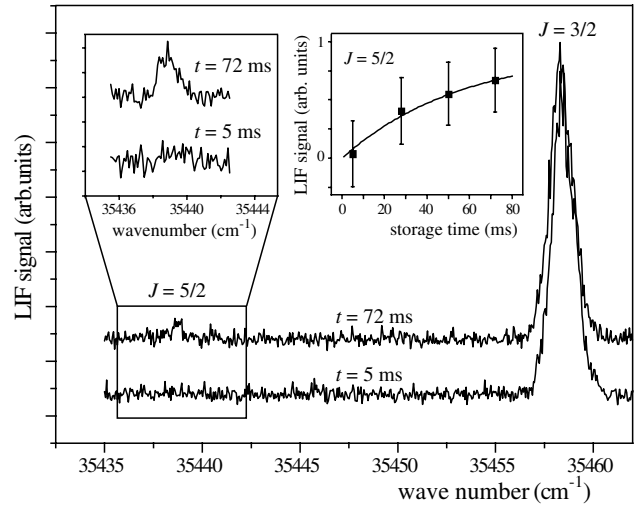
FIG. 3. Excitation spectrum of trapped OH ( v = 0 ) radicals that is recorded 5 ms (lower curve) and 72 ms (upper curve) after switching on the trap. In the central inset, the population of trapped OH radicals in the v = 0 , J = 5/2 level is shown as a function of the storage time.
