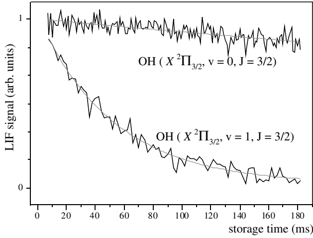
FIG. 2. Population of trapped OH radicals in the X^2\Pi_{3/2} , v = 0 , J = 3/2 level (upper curve) and in the X^2\Pi_{3/2} , v = 1 , J = 3/2 level (lower curve), as a function of the storage time t . The trapping potential is switched on at t = 0 ms.
