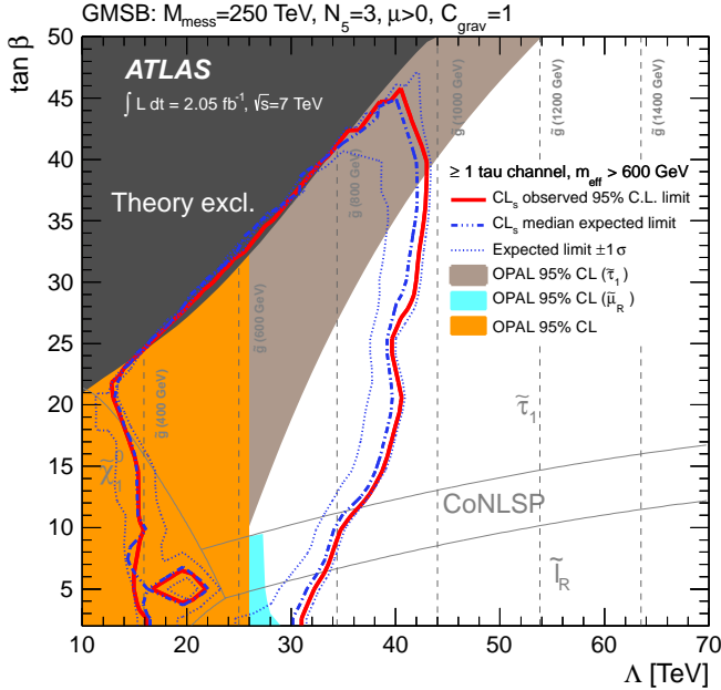
Figure 3: Expected and observed 95% C.L. exclusion limits in the M_{\text{mess}} = 250 \text{ TeV} , N_5 = 3 , \mu > 0 , C_{\text{grav}} = 1 slice of GMSB, together with the most stringent previous limits from OPAL [32]. The identity of the NLSP is indicated, with CoNLSP the region where the \tilde{\tau} and \tilde{\ell} are nearly degenerate.
