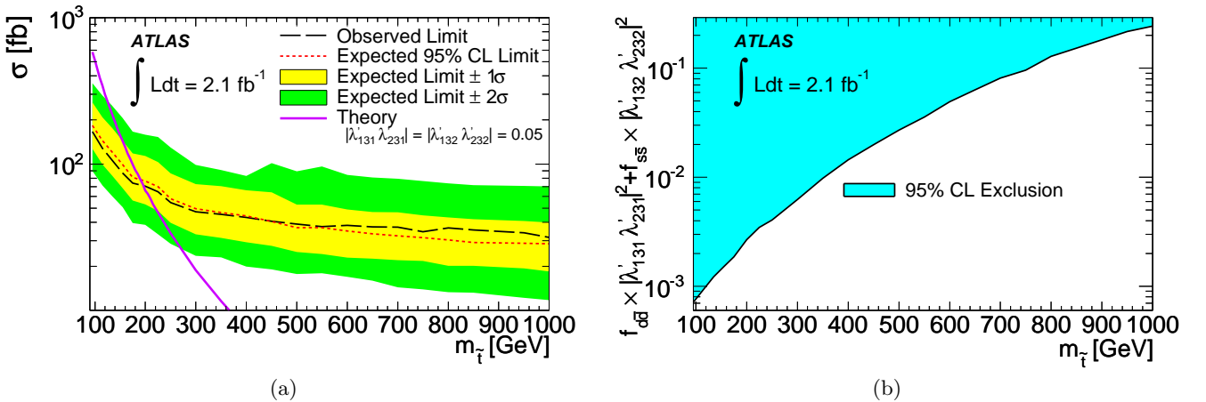
Fig. 4. (a) The observed 95% CL upper limits on \sigma(pp \rightarrow e\mu) through the t -channel exchange of a scalar top quark as a function of m_{\tilde{t}} . The expected limits are also shown together with the \pm 1 and \pm 2 standard deviation uncertainty bands. The theoretical cross section for |\lambda'_{131}\lambda_{231}| = |\lambda'_{132}\lambda_{232}| = 0.05 is also shown. (b) Excluded region for the PDF weighted sum of couplings ( f_{d\bar{d}} \times |\lambda'_{131}\lambda_{231}|^2 + f_{s\bar{s}} \times |\lambda'_{132}\lambda_{232}|^2 ) as a function of m_{\tilde{t}} .
