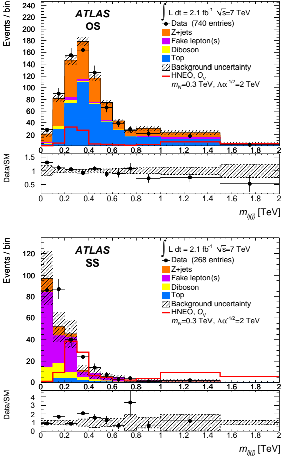
Fig. 1 Distributions of the reconstructed N invariant mass, m_{\ell\ell(j)} , for OS (top) and SS (bottom) dilepton events with \geq 1 jets and m_{\ell\ell} > 110 GeV. A selection criterion S_T \geq 400 GeV is used for the OS selection. The hypothetical signal distributions for m_N = 0.3 TeV for \mathcal{O}_V and \Lambda/\sqrt{\alpha}=2 TeV are superimposed.
