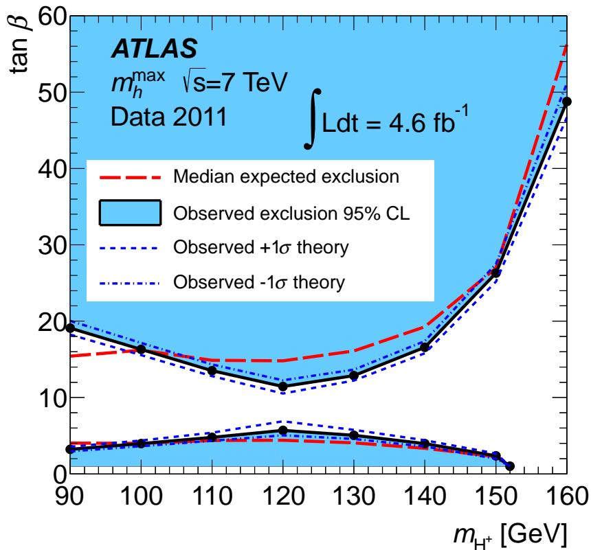
Figure 8. Combined 95% CL exclusion limits on \tan\beta as a function of m_{H^+} . Results are shown in the context of the MSSM scenario m_h^{\max} for the region 1 < \tan\beta < 60 in which reliable theoretical predictions exist. The theoretical uncertainties described in the text are shown as well.
