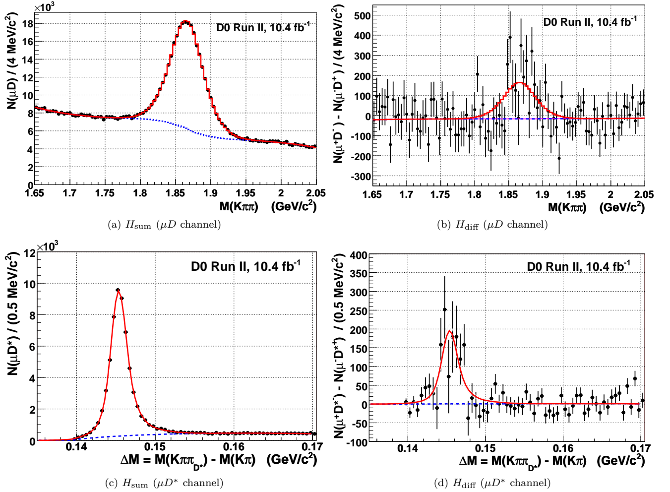
FIG. 3: Examples of the raw asymmetry fit for the two decay channels, for the fifth \text{VPDL}(B^0) bin corresponding to (0.10 < \text{VPDL}(B^0) < 0.20) cm. The left plots show the sum distributions; the right plots show the difference distributions. In both cases, the solid line represents the total fit function, with the background part shown separately by the dashed line (see text).
