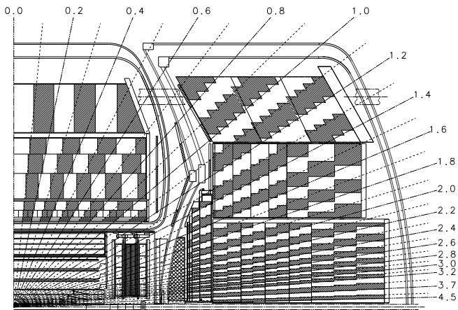
FIG. 1. One quadrant of the DØ calorimeter and drift chambers, projected in the r - z plane. Radial lines illustrate the detector pseudorapidity and the pseudo-projective geometry of the calorimeter towers. Each tower has size \Delta\eta \times \Delta\phi = 0.1 \times 0.1 .
