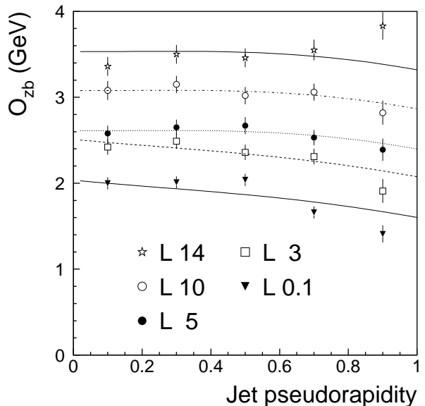
FIG. 7. The offset correction O_{\text{zb}} as a function of pseudorapidity of k_{\perp} jet ( D = 1.0 ). The offset O_{\text{zb}} accounts for the combined effects of pile-up, uranium noise, and multiple interactions. The different sets of points are for events with different instantaneous luminosities \mathcal{L} \approx 14, 10, 5, 3, 0.1 \times 10^{30} \text{cm}^{-2} \text{s}^{-1} . The curves are fits to the points at different \mathcal{L} , using the same functional form as employed for the cone algorithm in Ref. [35].
