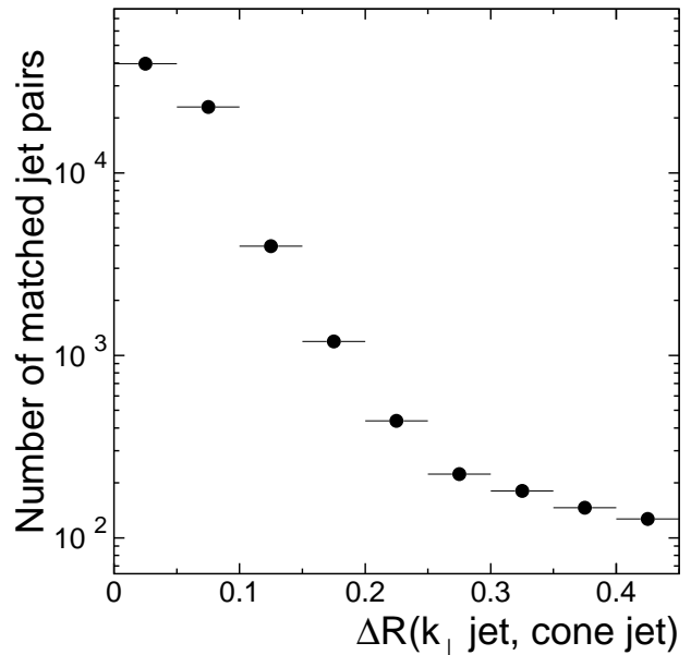
FIG. 10. The distance \Delta\mathcal{R} = \sqrt{\Delta\eta^2 + \Delta\phi^2} between a k_{\perp} -jet axis and its matching cone-jet axis. The k_{\perp} jets were reconstructed with D = 1.0 , and the cone jets were reconstructed with \mathcal{R} = 0.7 . Only the two leading jets from each algorithm were considered. The k_{\perp} jets were selected with |\eta| < 0.5 .
