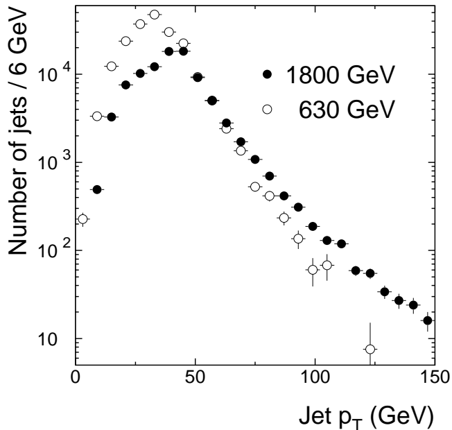
FIG. 13. The p_T distribution of selected central ( |\eta| < 0.5 ) jets in D\bar{O} data, before applying a cutoff on jet p_T . The data at \sqrt{s} = 630 GeV are normalized to the data at \sqrt{s} = 1800 GeV in the bin 54 \leq p_T < 60 GeV. The turnover at lower jet p_T is due to inefficiencies in the trigger. For the following analysis, we use jets with 55 < p_T < 100 GeV.
