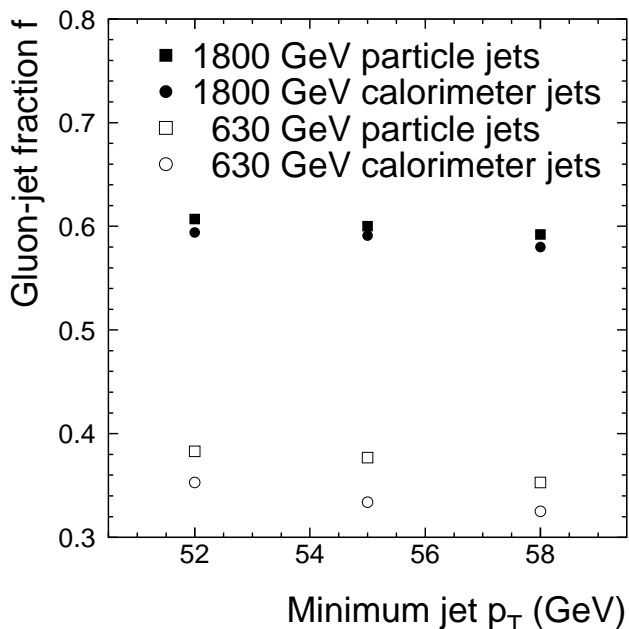
FIG. 16. The gluon-jet fraction of selected jets with maximum p_T = 100 GeV and minimum p_T between 52 and 58 GeV, as a function of minimum jet p_T , for \sqrt{s} = 1800 GeV and 630 GeV, using the CTEQ4M PDF. The jets have been tagged through the identity of the nearer leading-order final-state parton.
