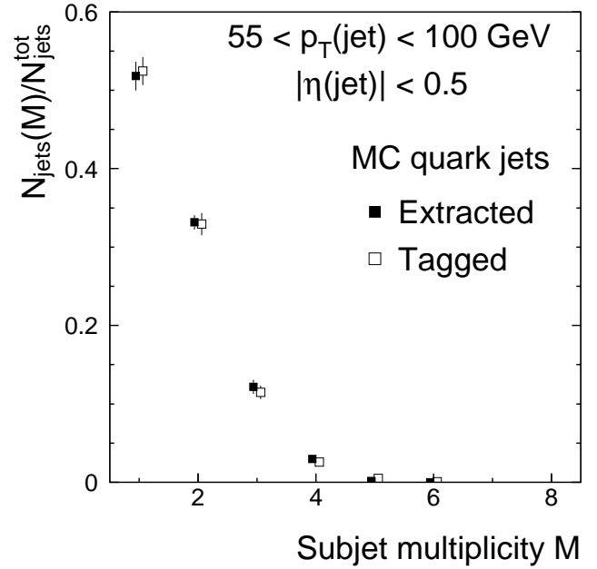
FIG. 28. The subjet multiplicity in Monte Carlo quark jets. The extracted distribution has been unsmeared. The tagged distribution was obtained directly from particle-level quark jets at \sqrt{s} = 1800 GeV.
