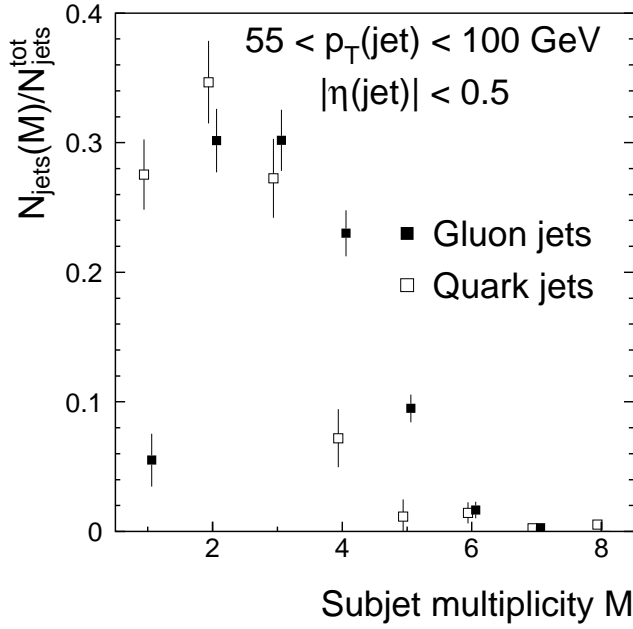
FIG. 22. Uncorrected subjet multiplicity in gluon and quark jets, extracted from D\bar{O} data at \sqrt{s} = 1800 GeV and 630 GeV, using nominal gluon-jet fractions f_{1800} = 0.59 and f_{630} = 0.33 .
