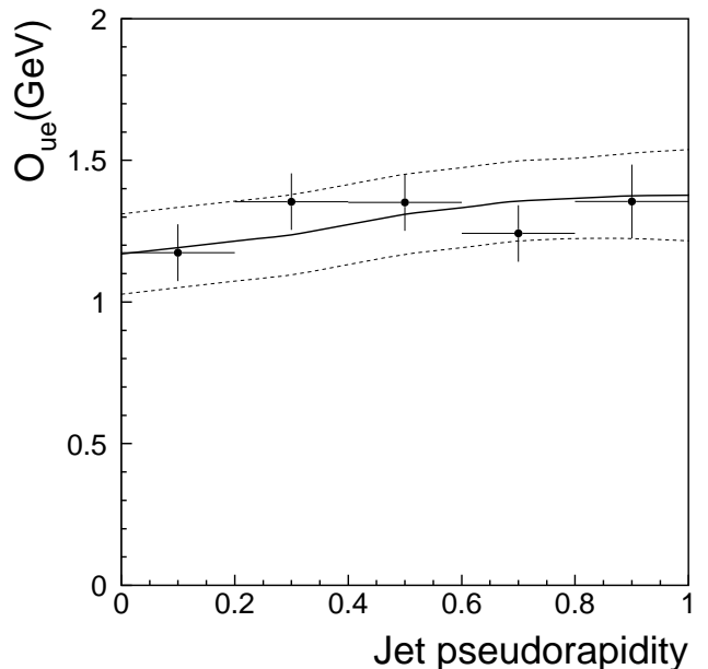
FIG. 8. The correction for underlying event O_{ue} as a function of |\eta| for k_{\perp} jets ( D = 1.0 ). The solid curve is the fit of the results for the cone jet algorithm in Ref. [35] scaled to the results for the k_{\perp} jet algorithm. The dashed curves denote the one standard deviation (s.d.) systematic error.
