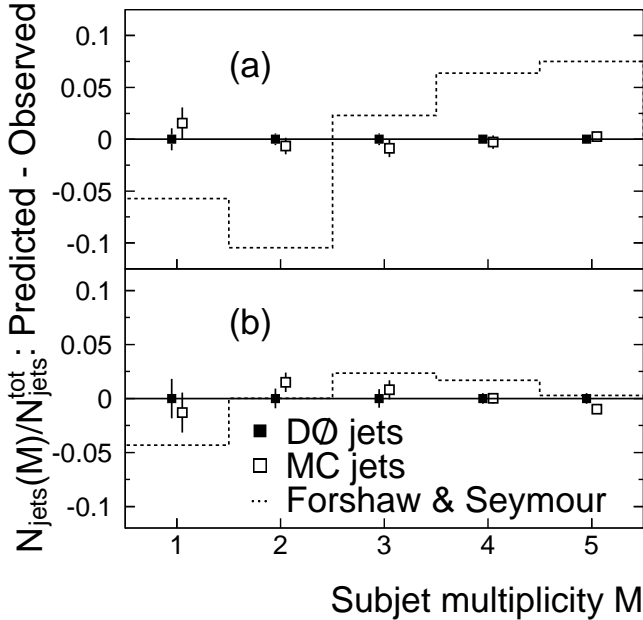
FIG. 30. The subject multiplicity in gluon and quark jets, for y_{\text{cut}} = 10^{-3} (as defined by Eq. [3.6]), in a resummation calculation by Forshaw and Seymour [17]. The jets are produced at \sqrt{s} = 1800 GeV, with p_T = 65 GeV and \eta = 0 , using the CTEQ4M PDF, and are reconstructed with D = 0.5 . The points in the fifth bin refer to M \geq 5 .
