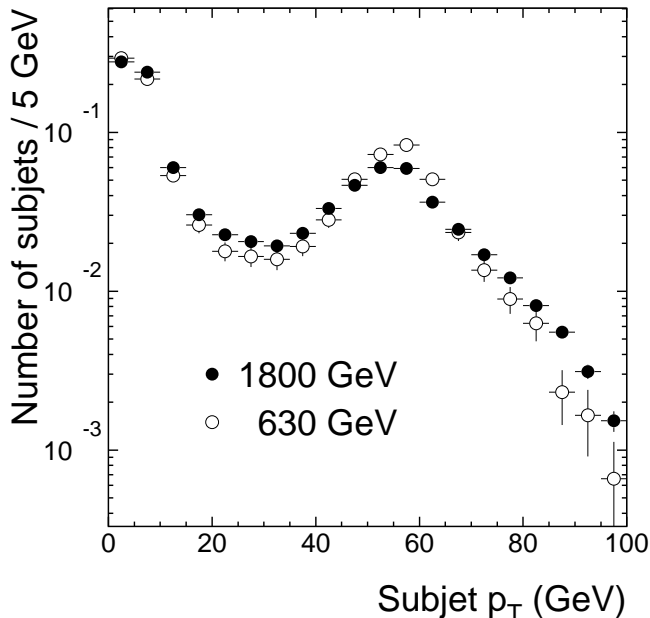
FIG. 20. The uncorrected p_T distribution of subjects in data for jets with 55 < p_T < 100 GeV and |\eta| < 0.5 . All selections have been applied, and each distribution has been normalized to unit area.
