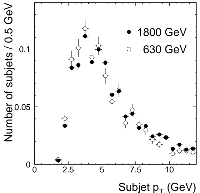
FIG. 21. Same as in Fig. 20, but with the low p_T region expanded. The increase at low p_T is observed for all y_{\text{cut}} , but the specific cutoff at p_T(\text{subject}) \approx 1.75 GeV is determined by our chosen value of y_{\text{cut}} = 10^{-3} .
