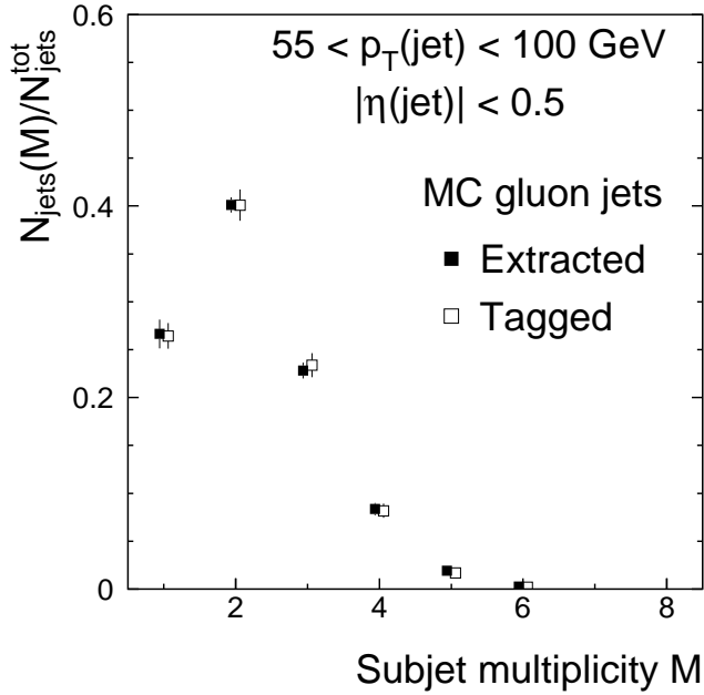
FIG. 27. The subjet multiplicity in Monte Carlo gluon jets. The extracted distribution has been unsmeared. The tagged distribution was obtained directly from particle-level gluon jets at \sqrt{s} = 1800 GeV.
