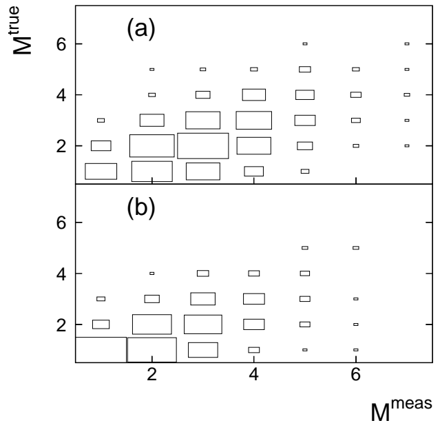
FIG. 26. The subject multiplicity at particle-level ( M^{\text{true}} ) versus the subject multiplicity at calorimeter-level ( M^{\text{meas}} ) (includes effects of luminosity), at \sqrt{s} = 1800 GeV, for (a) gluon and (b) quark jets.
