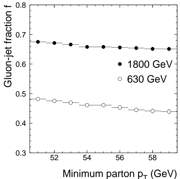
FIG. 12. The Monte Carlo gluon-jet fraction f at leading-order, for final-state partons with maximum parton p_T = 100 GeV, and minimum parton p_T \approx 55 GeV, as a function of the minimum parton p_T , using the CTEQ4M PDF. Both partons are required to be central ( |\eta| < 0.5 ). The solid symbols show the prediction for \sqrt{s} = 1800 GeV, and the open symbols show the prediction for \sqrt{s} = 630 GeV.
