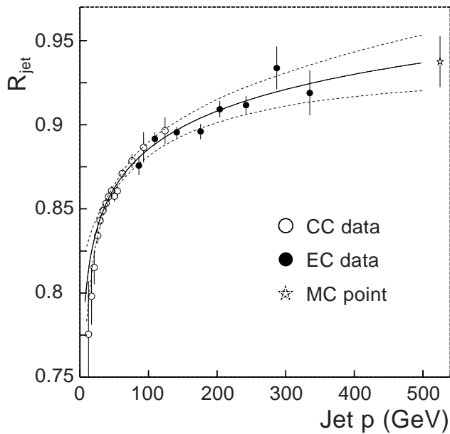
FIG. 9. The response correction for k_{\perp} jets with D = 1.0 , as a function of offset-corrected jet momentum. The Monte Carlo point ( \star ) is used to constrain the fit (solid) at high p_{\text{jet}}^{\text{meas}} . The dashed curves denote the \pm 1 s.d. systematic error.
