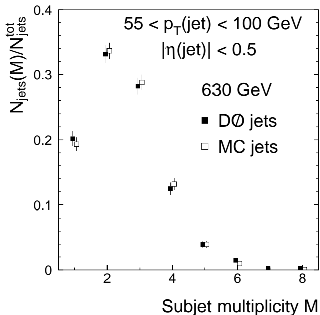
FIG. 25. Uncorrected subject multiplicity in jets from D\bar{D} and from fully-simulated Monte Carlo events at \sqrt{s} = 630 GeV.
