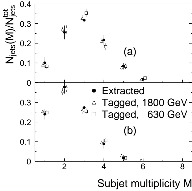
FIG. 17. Uncorrected subjet multiplicity in fully-simulated Monte Carlo (a) gluon and (b) quark jets. The number of jets N_{\text{jets}}(M) in each bin of subjet multiplicity on the vertical axis is normalized to the total number of jets in each sample N_{\text{jets}}^{\text{tot}} = \sum_M N_{\text{jets}}(M) . The measured distributions (solid) are extracted from the mixed Monte Carlo jet samples at \sqrt{s} = 1800 GeV and 630 GeV. The tagged distributions (open) are for \sqrt{s} = 1800 GeV (triangles) and 630 GeV (squares).
