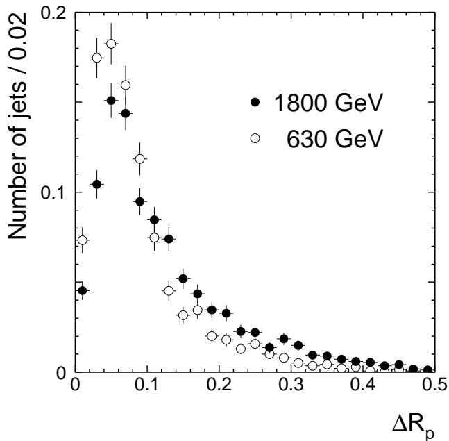
FIG. 15. The distance of the closest calorimeter-level Monte Carlo jet to one of the leading final-state partons. The solid (open) points show the Monte Carlo sample at \sqrt{s} = 1800 (630) GeV. Each distribution has been normalized to unit area.
