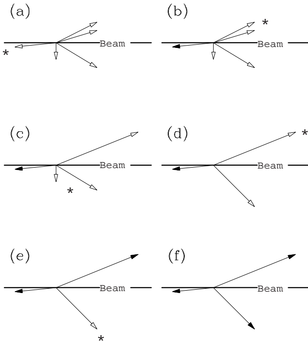
FIG. 4. A simplified example of the final state of a collision between two hadrons. (a) The particles in the event (represented by arrows) comprise a list of objects. (b-f) Solid arrows represent the final jets reconstructed by the k_{\perp} algorithm, and open arrows represent objects not yet assigned to jets. The five diagrams show successive iterations of the algorithm. In each diagram, a jet is either defined (when it is well-separated from all other objects), or two objects are merged (when they have small relative k_{\perp} ). The asterisk labels the relevant object(s) at each step.
