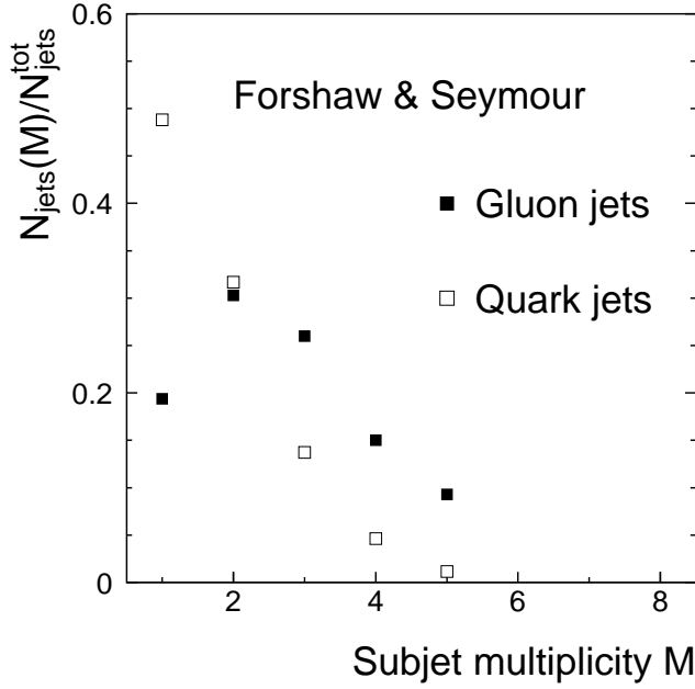
FIG. 30. The subject multiplicity in gluon and quark jets, for y_{\text{cut}} = 10^{-3} (as defined by Eq. [3.6]), in a resummation calculation by Forshaw and Seymour [17]. The jets are produced at \sqrt{s} = 1800 GeV, with p_T = 65 GeV and \eta = 0 , using the CTEQ4M PDF, and are reconstructed with D = 0.5 . The points in the fifth bin refer to M \geq 5 .
