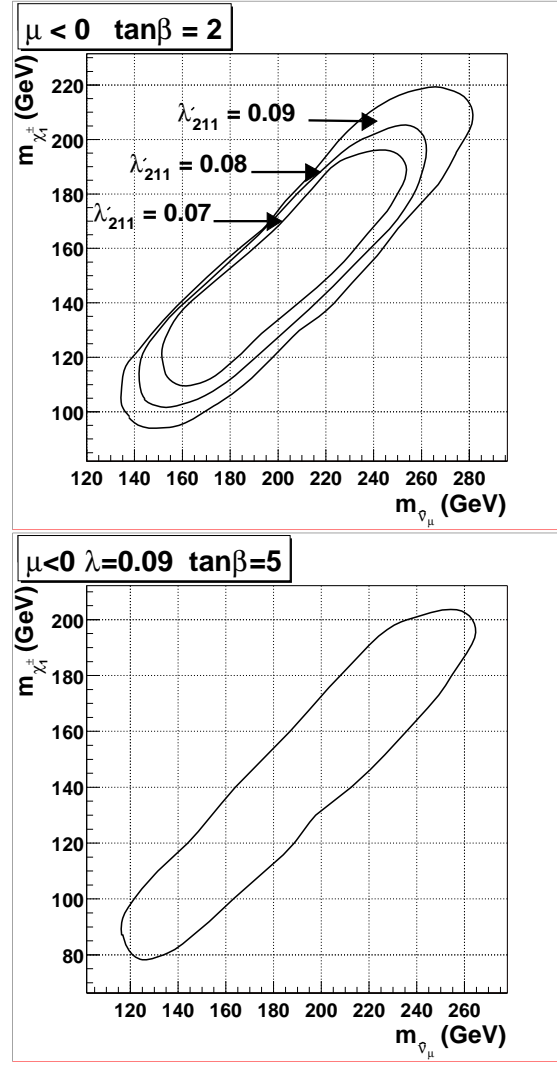
FIG. 2. Exclusion contours at the 95% C.L. in the (m_{\tilde{\nu}_\mu}/m_{\tilde{\nu}}, m_{\chi^+}) plane. The top figure is for \tan\beta = 2 , and three values of \lambda'_{211} , while the bottom figure is for \tan\beta = 5 and \lambda'_{211} = 0.09 . We give all contour plots as a function of the sneutrino mass. Because, for any given set of parameters, the sneutrino mass is very close to the smuon mass, the smuon contour plots lie very close to the sneutrino results, and are therefore not shown.
