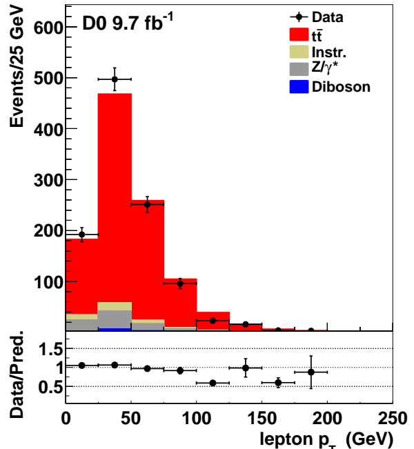
FIG. 1: The distributions in lepton p_T and the ratio of data to predictions for the combined ee , e\mu , and \mu\mu final states after applying requirements (i) – (vii).
